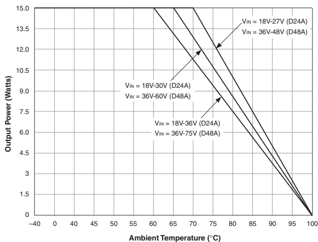
D24A and D48A Temperature Derating for 2.5/5/12/15V Output Models
