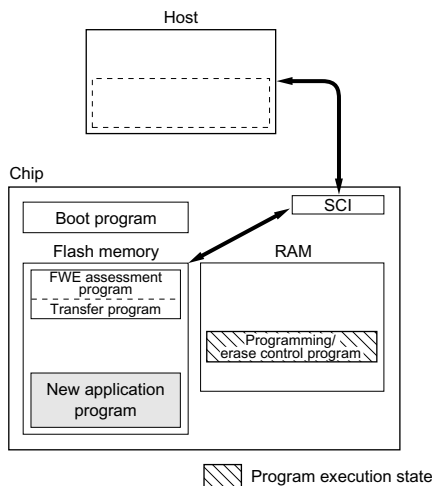
Figure 19-62 User Program Mode (Example)
