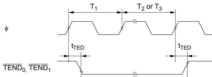
Figure 22-18 DMAC \overline{TEND} Output Timing
