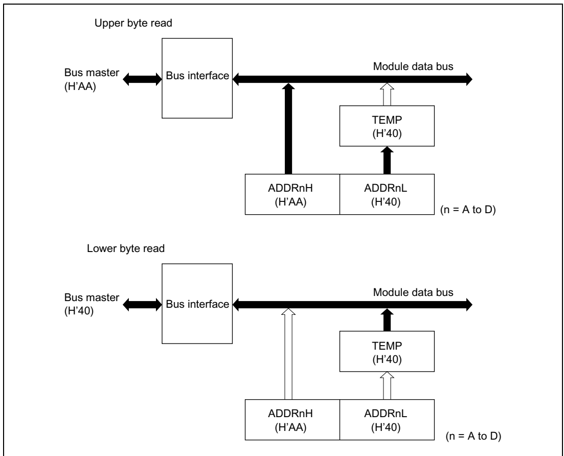
Figure 16-2 ADDR Access Operation (Reading H'AA40)
