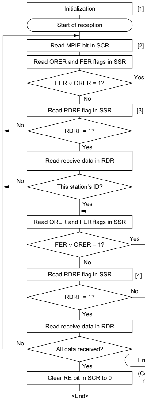
Figure 14-12 Sample Multiprocessor Serial Reception Flowchart
