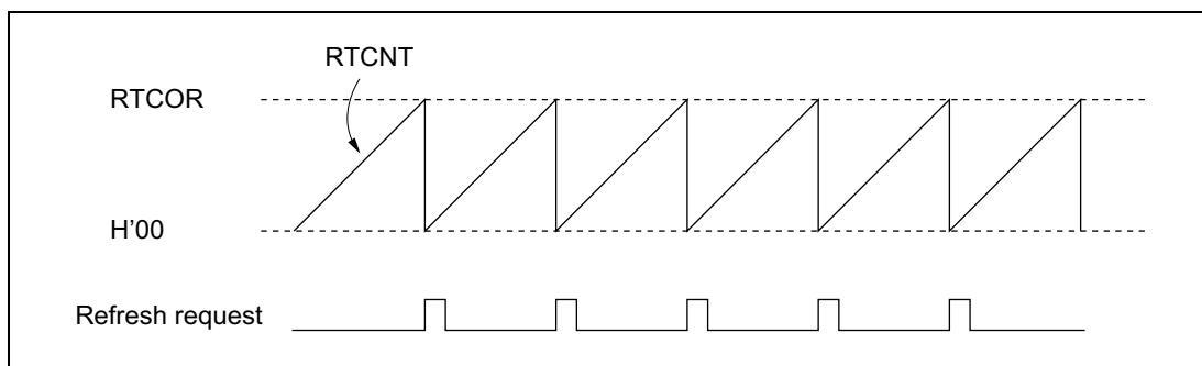
Figure 6-23 RTCNT Operation
