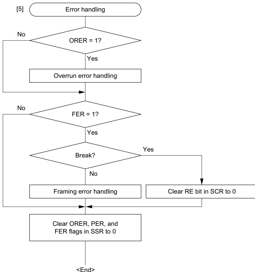
Figure 14-12 Sample Multiprocessor Serial Reception Flowchart (cont)
