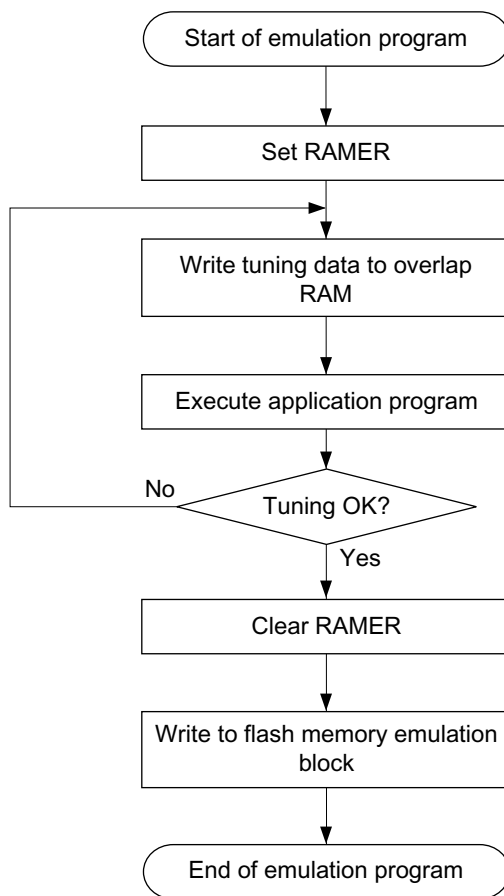
Figure 19-17 Flowchart for Flash Memory Emulation in RAM
