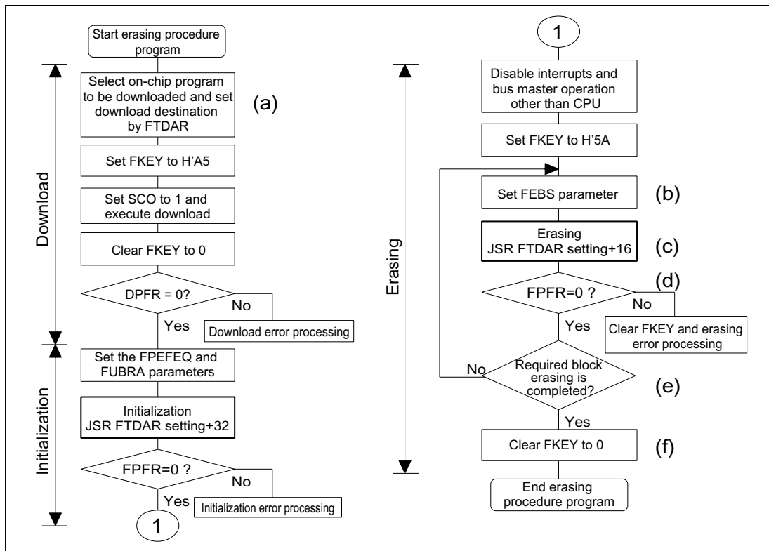
Figure 19-100 Erasing Procedure
