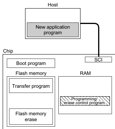
Figure 19-5 User Program Mode (Example)
