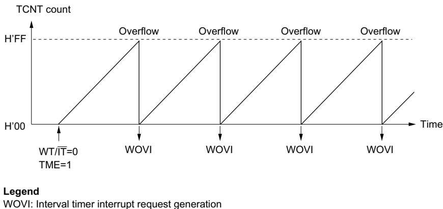
Figure 13-5 Operation in Interval Timer Mode
