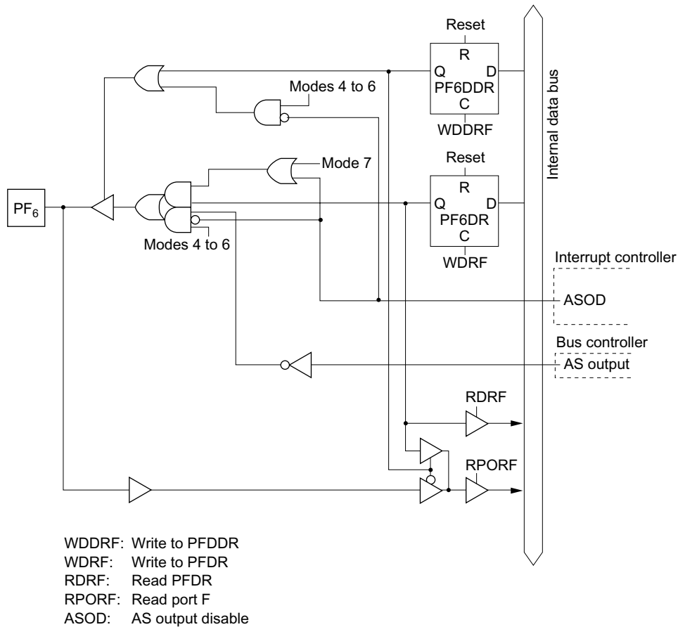
Figure C-12 (g) Port F Block Diagram (Pin PF 6 )
