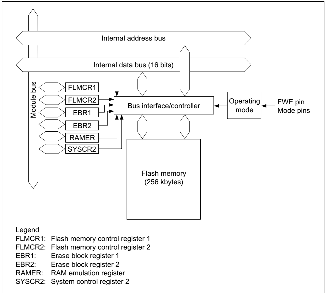
Figure 19-29 Block Diagram of Flash Memory
