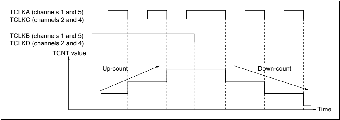
Figure 10-30 Example of Phase Counting Mode 2 Operation
