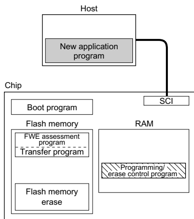
Figure 19-32 User Program Mode (Example)
