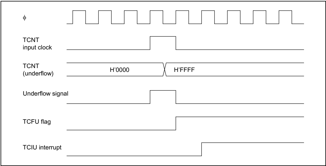
Figure 10-45 TCIU Interrupt Setting Timing
