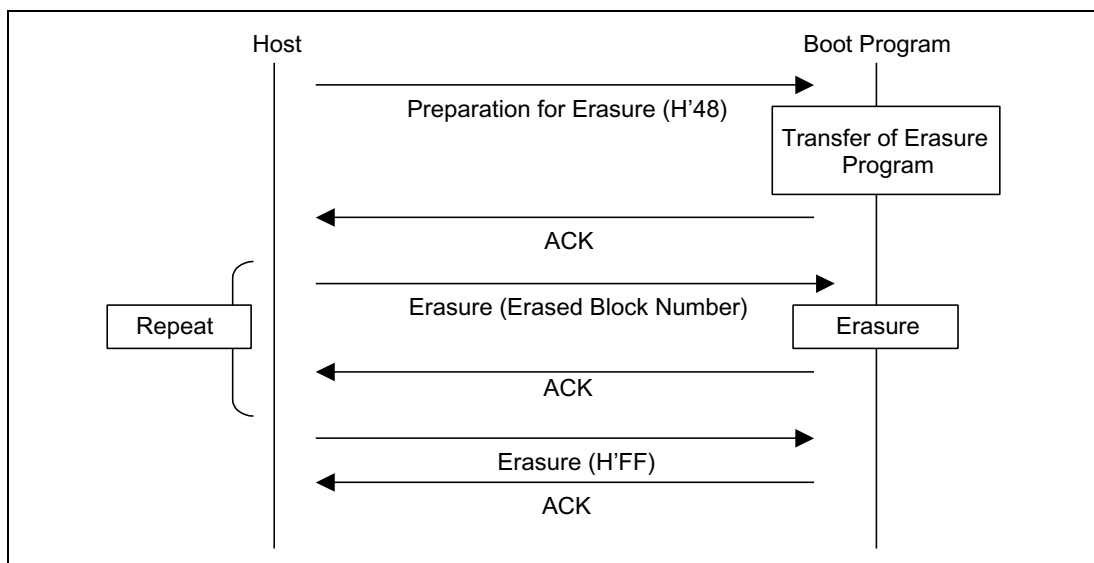
Figure 19-116 Erasure Sequence
