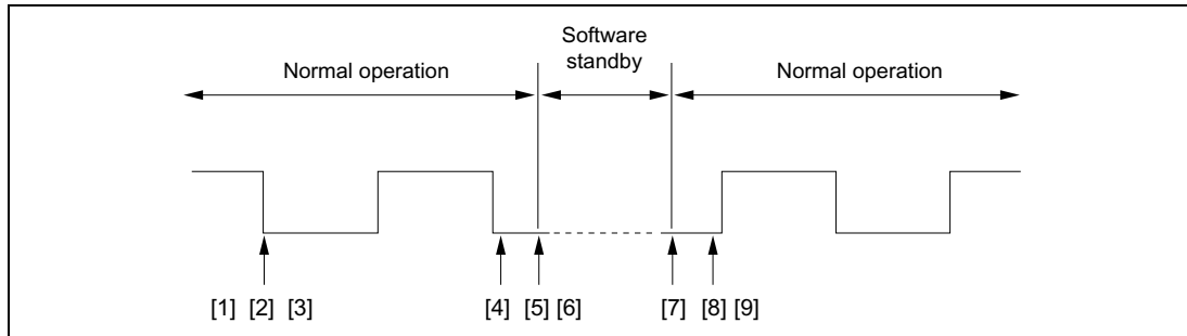
Figure 15-9 Clock Halt and Restart Procedure
