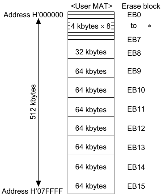
Figure 19-92 Block Division of User MAT
