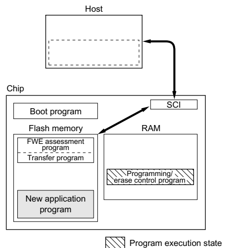
Figure 19-32 User Program Mode (Example)
