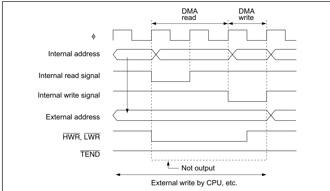
Figure 7-42 Example in Which Low Level is Not Output at \overline{TEND} Pin
