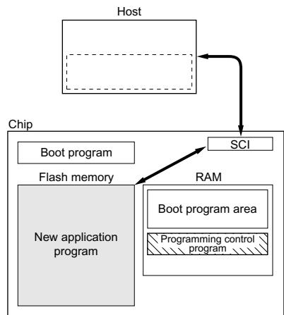
Figure 19-61 Boot Mode
