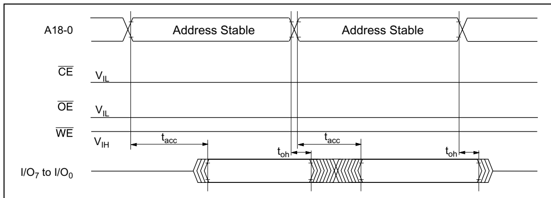
Figure 19-119 \overline{\text{CE}}/\overline{\text{OE}} Enable State Read
