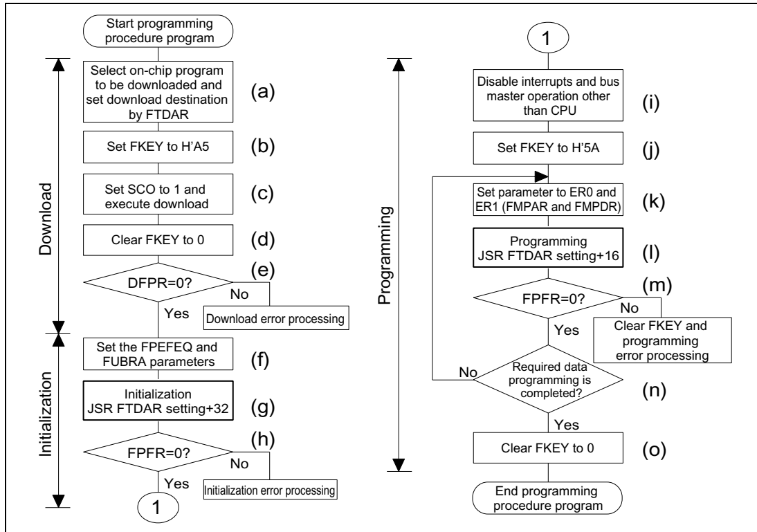
Figure 19-99 Programming Procedure
