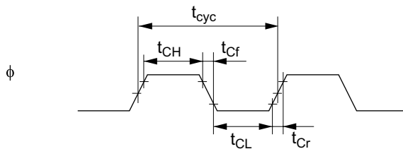
Figure 22-2 System Clock Timing
