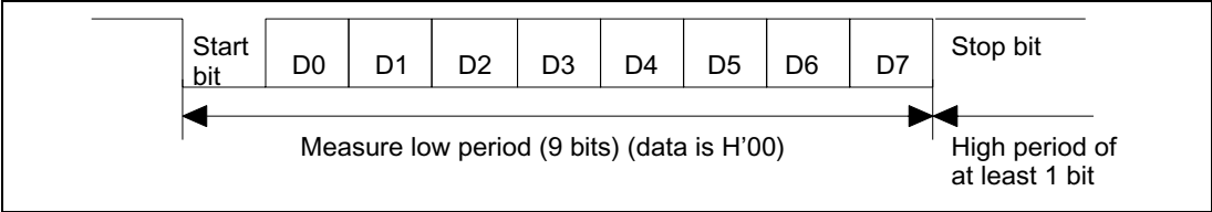
Figure 19-95 Automatic Adjustment Operation of SCI Bit Rate
