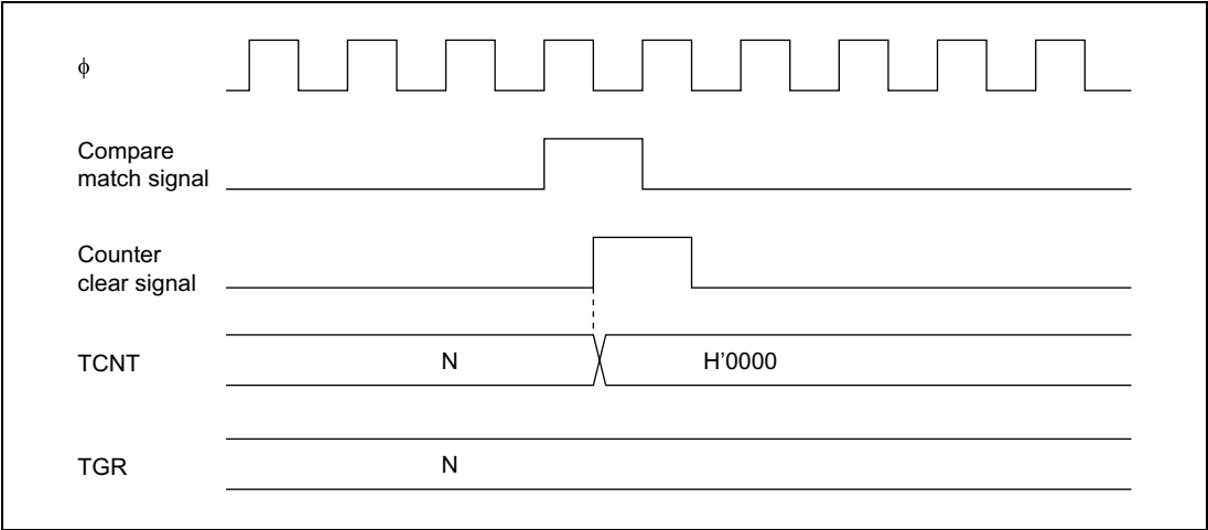
Figure 10-38 Counter Clear Timing (Compare Match)
