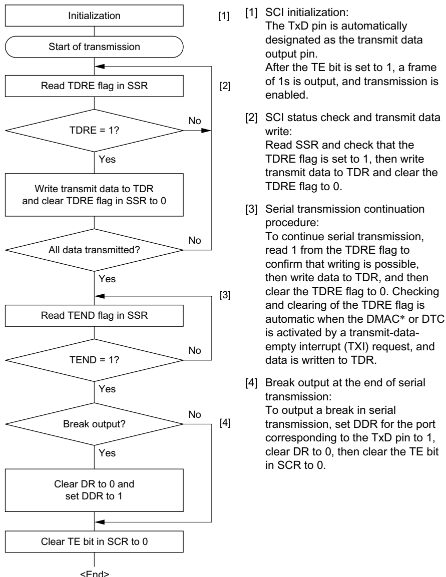
Figure 14-5 Sample Serial Transmission Flowchart
