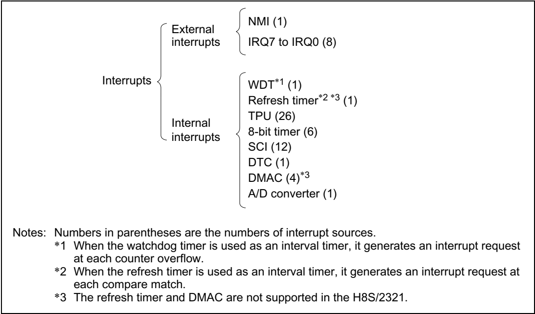
Figure 4-3 Interrupt Sources and Number of Interrupts
