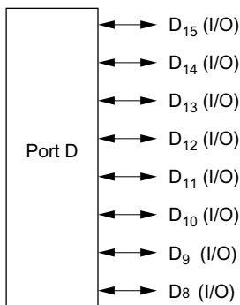
Figure 9-17 Port D Pin Functions (Modes 4 to 6)
