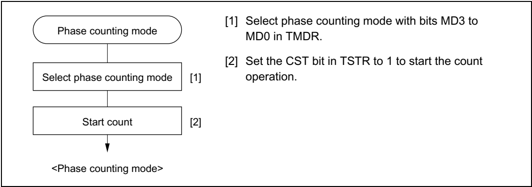
Figure 10-28 Example of Phase Counting Mode Setting Procedure
