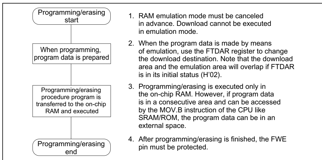
Figure 19-97 Programming/Erasing Overview Flow
