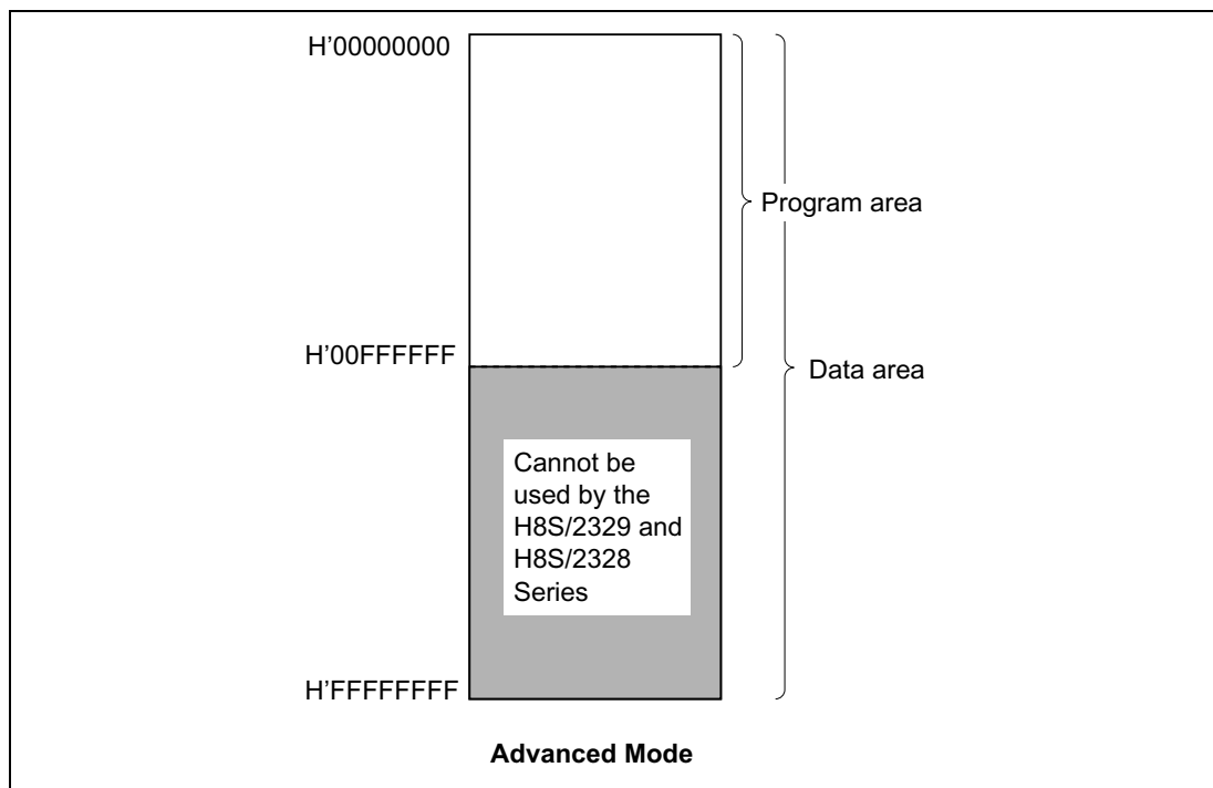
Figure 2-3 Memory Map
