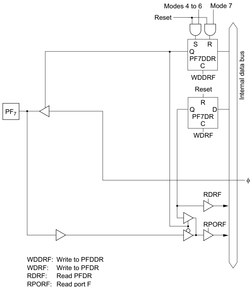
Figure C-12 (h) Port F Block Diagram (Pin PF 7 )
