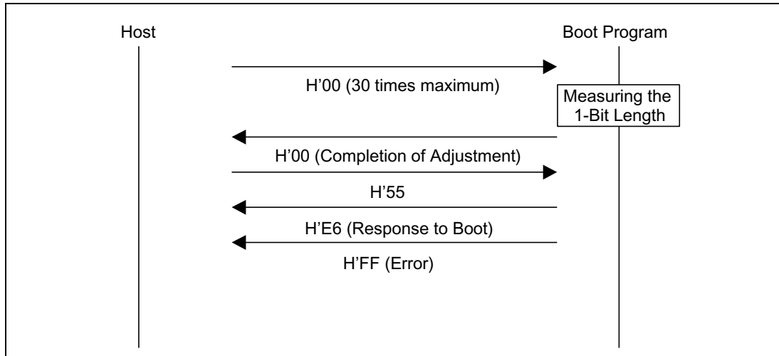
Figure 19-112 Bit-Rate-Adjustment Sequence
