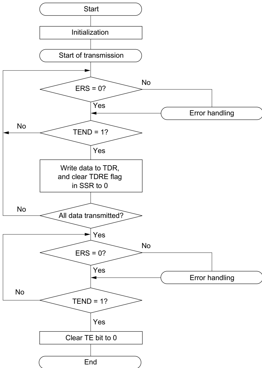
Figure 15-4 Sample Transmission Flowchart
