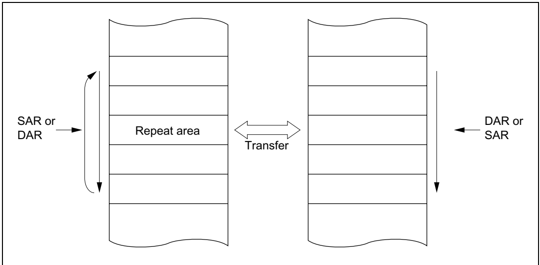
Figure 8-7 Memory Map in Repeat Mode
