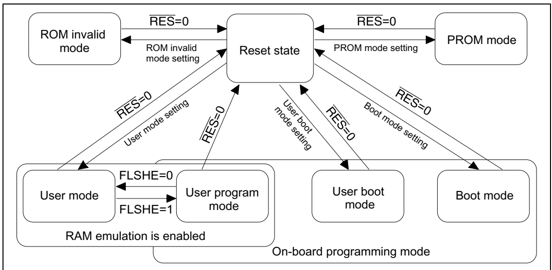
Figure 19-90 Mode Transition of Flash Memory
