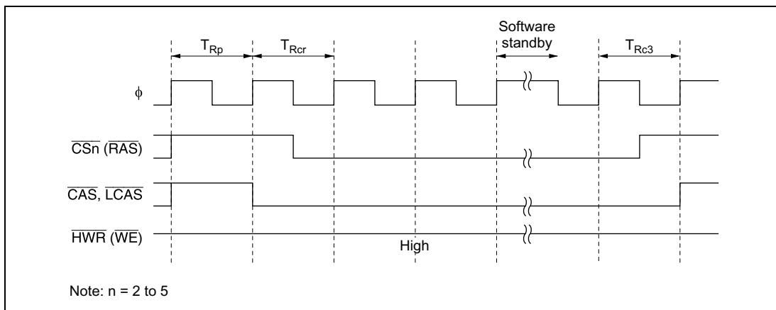
Figure 6-27 Self-Refresh Timing
