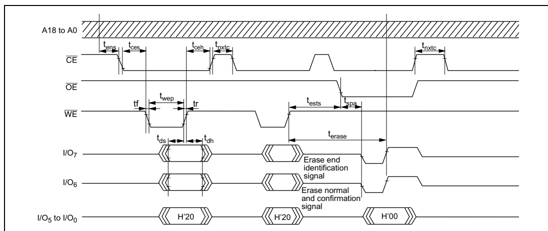
Figure 19-122 Timing in Auto-Erase Mode
