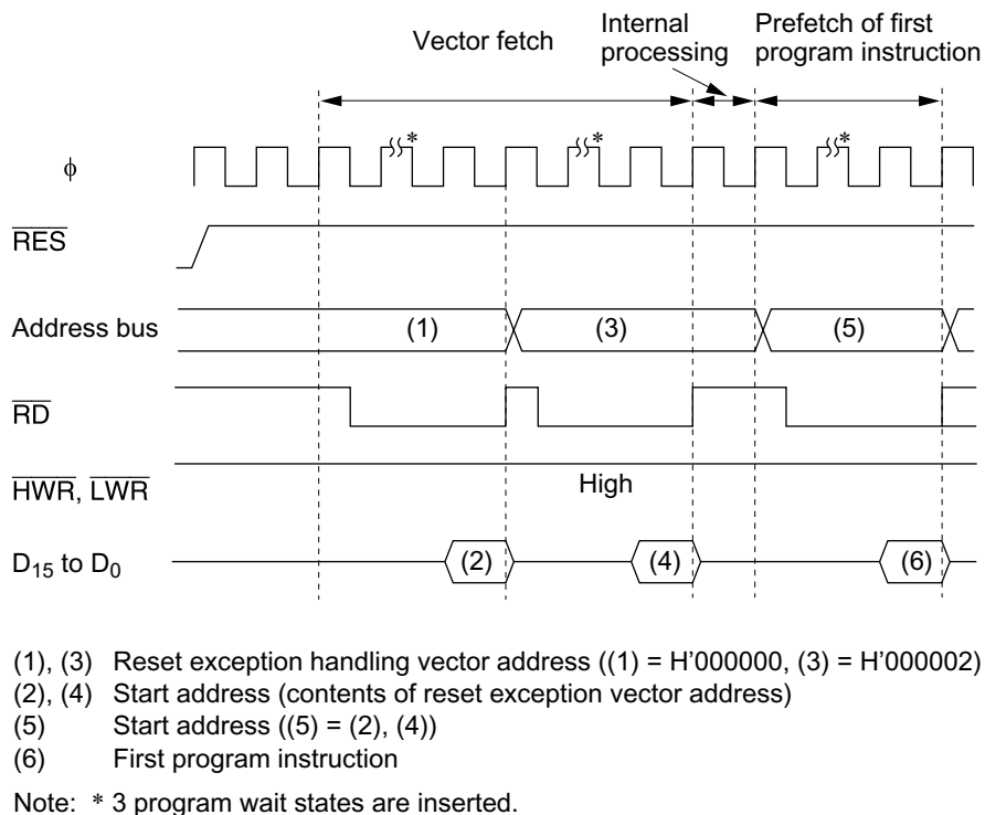
Figure 4-2 Reset Sequence (Mode 4)
