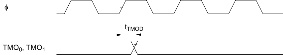
Figure 22-24 8-Bit Timer Output Timing
