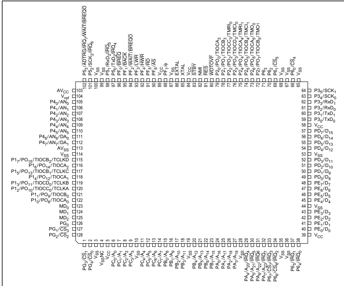
Figure 1-6 H8S/2321 Pin Arrangement (FP-128B: Top View)
