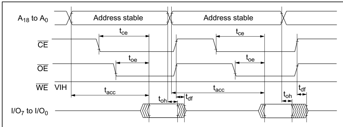
Figure 19-51 Timing Waveforms for \overline{\text{CE}}/\overline{\text{OE}} Clocked Read
