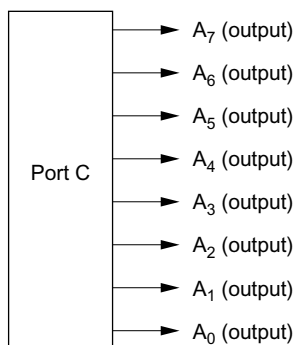
Figure 9-13 Port C Pin Functions (Modes 4 and 5)
