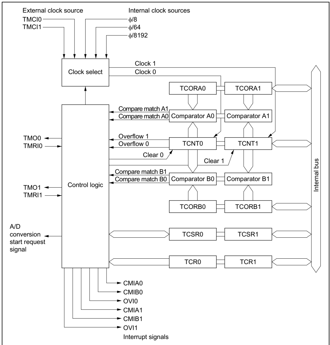
Figure 12-1 Block Diagram of 8-Bit Timer Module
