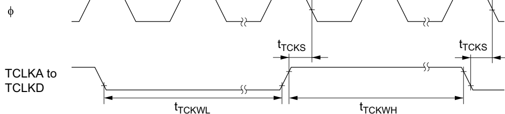
Figure 22-23 TPU Clock Input Timing
