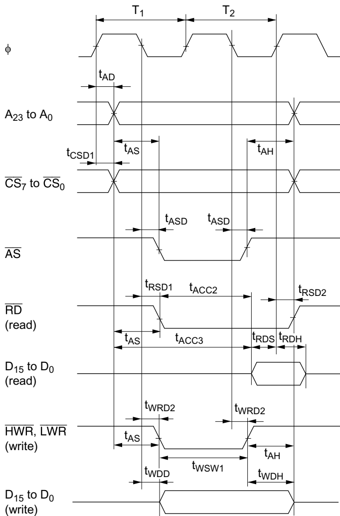
Figure 22-6 Basic Bus Timing (2-State Access)
