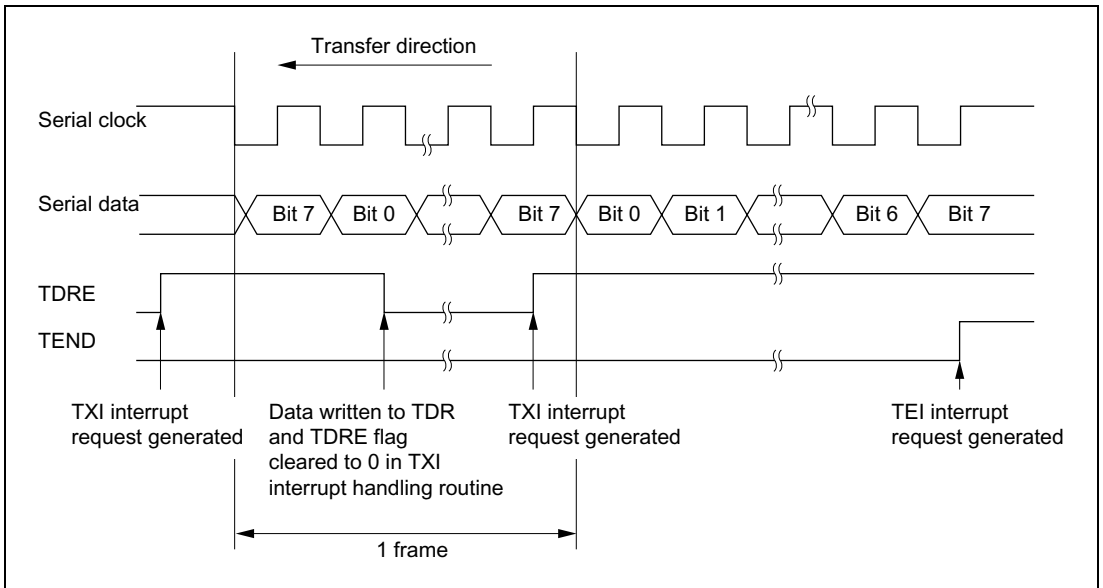
Figure 14-17 Example of SCI Transmit Operation
