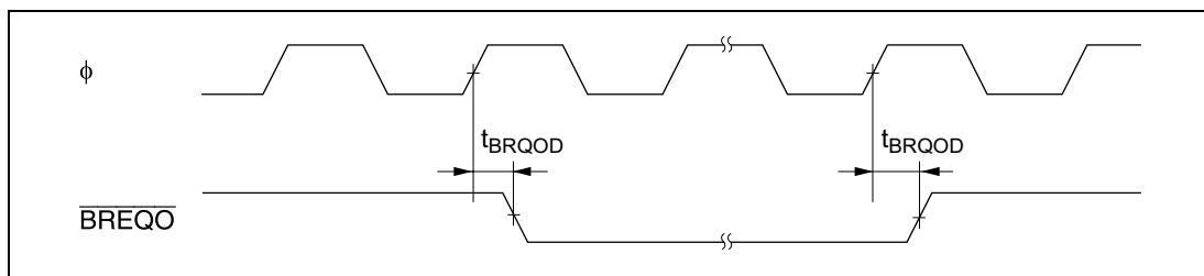
Figure 22-15 External Bus Request Output Timing
