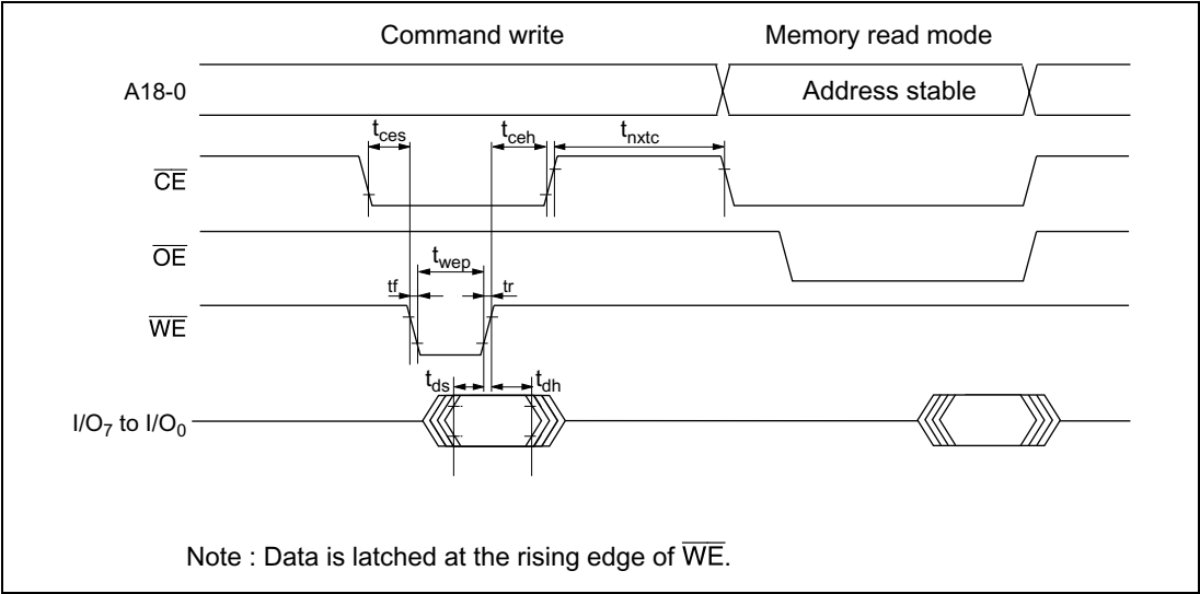
Figure 19-117 Memory Read Timing after Command Write
