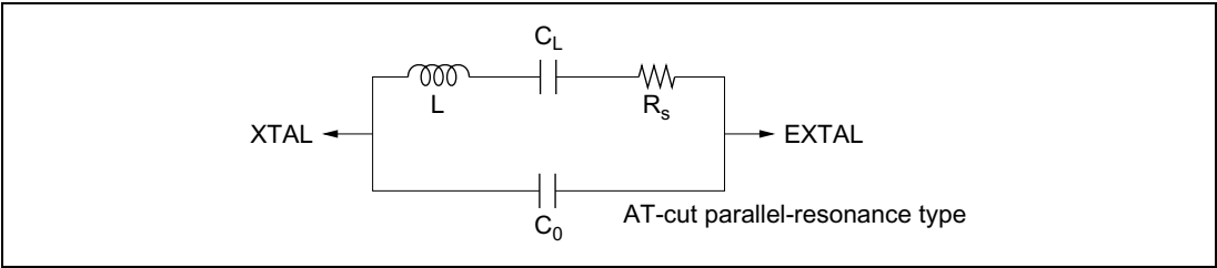
Figure 20-3 Crystal Resonator Equivalent Circuit
