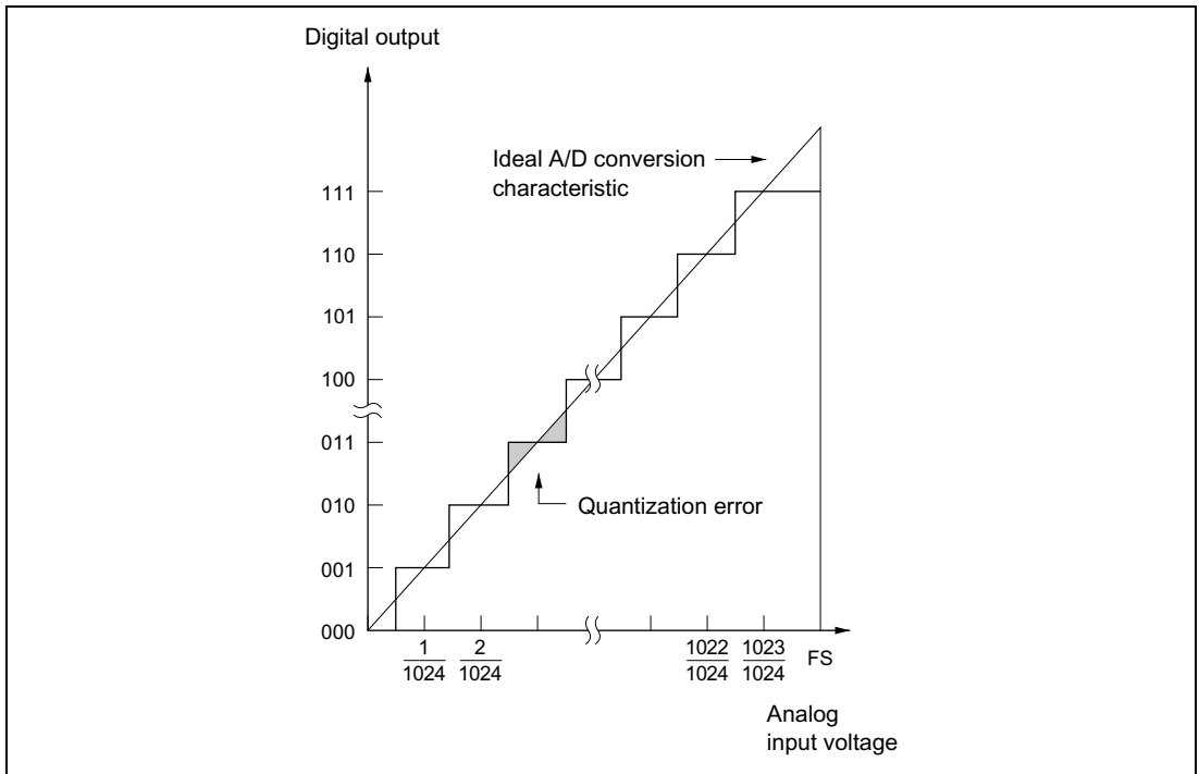
Figure 16-8 A/D Conversion Precision Definitions (1)
