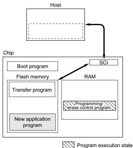
Figure 19-5 User Program Mode (Example)
