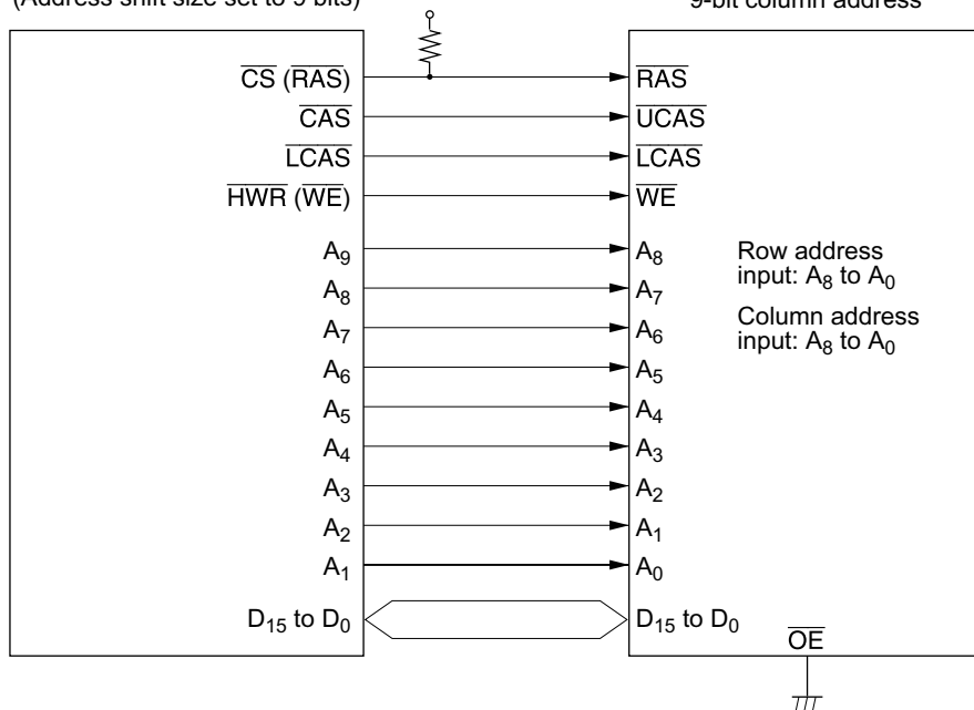
Figure 6-19 Example of 2-CAS DRAM Connection
