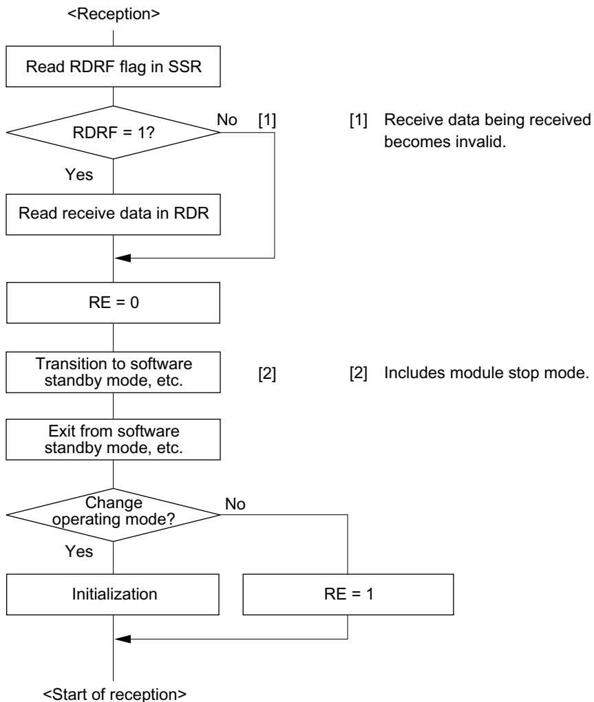
Figure 14-26 Sample Flowchart for Mode Transition during Reception
