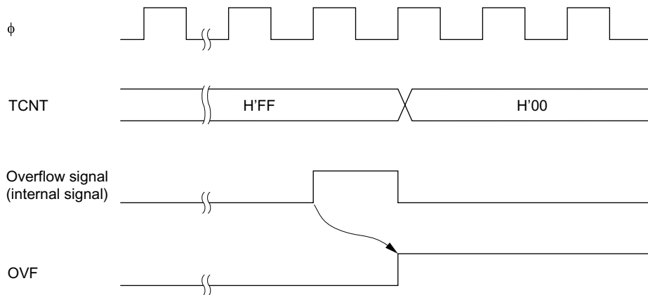
Figure 13-6 Timing of OVF Setting
