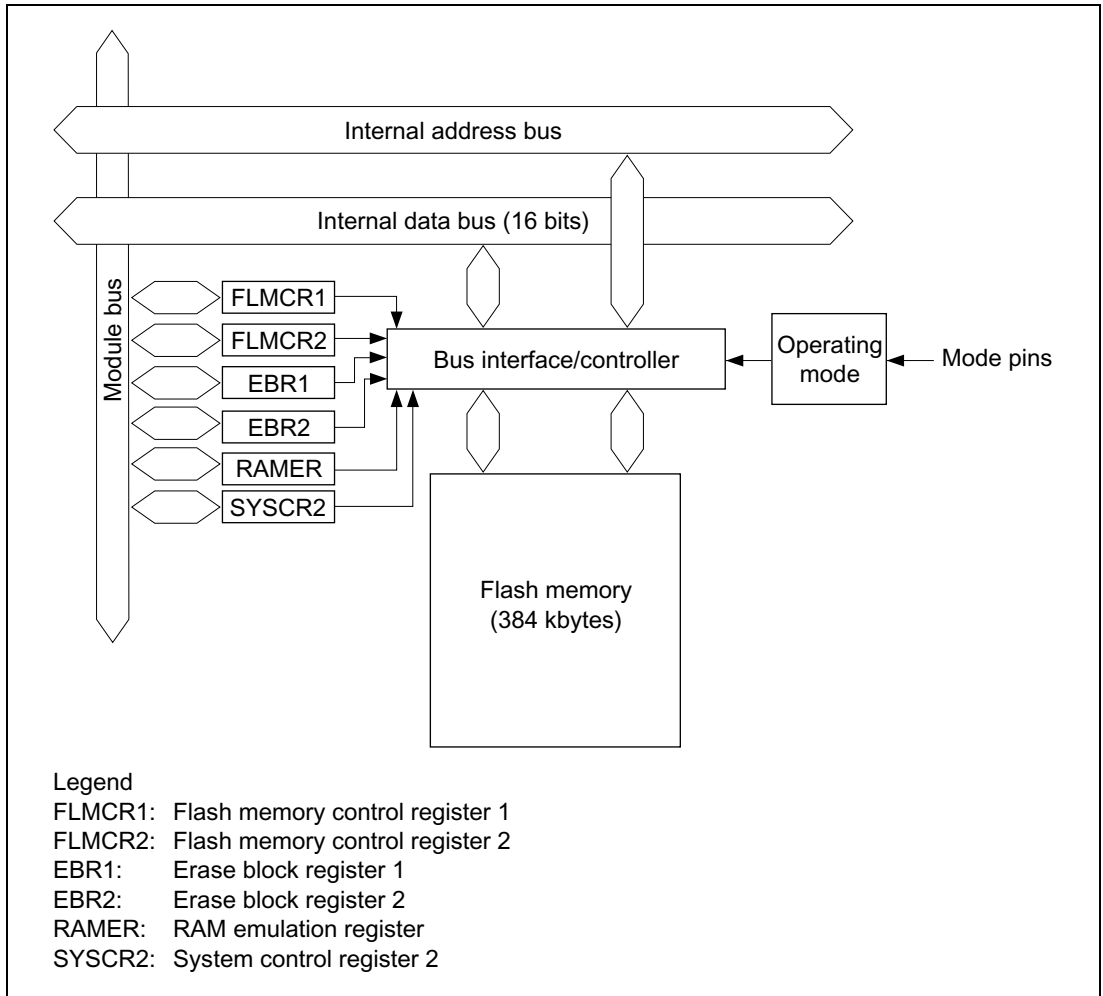
Figure 19-2 Block Diagram of Flash Memory
