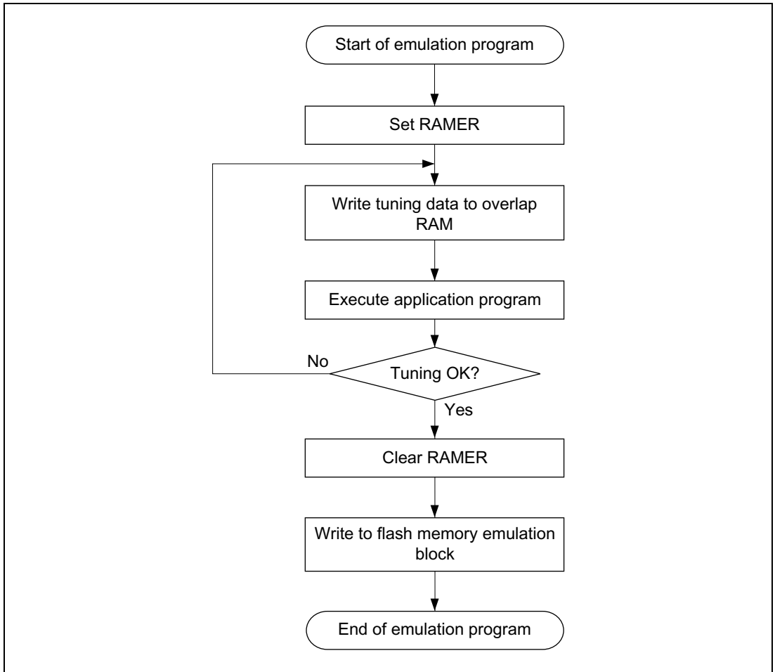
Figure 19-74 Flowchart for Flash Memory Emulation in RAM
