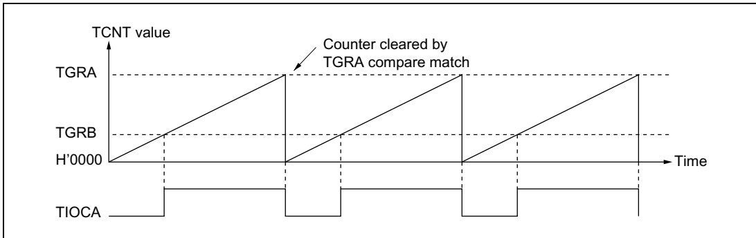
Figure 10-25 Example of PWM Mode Operation (1)
