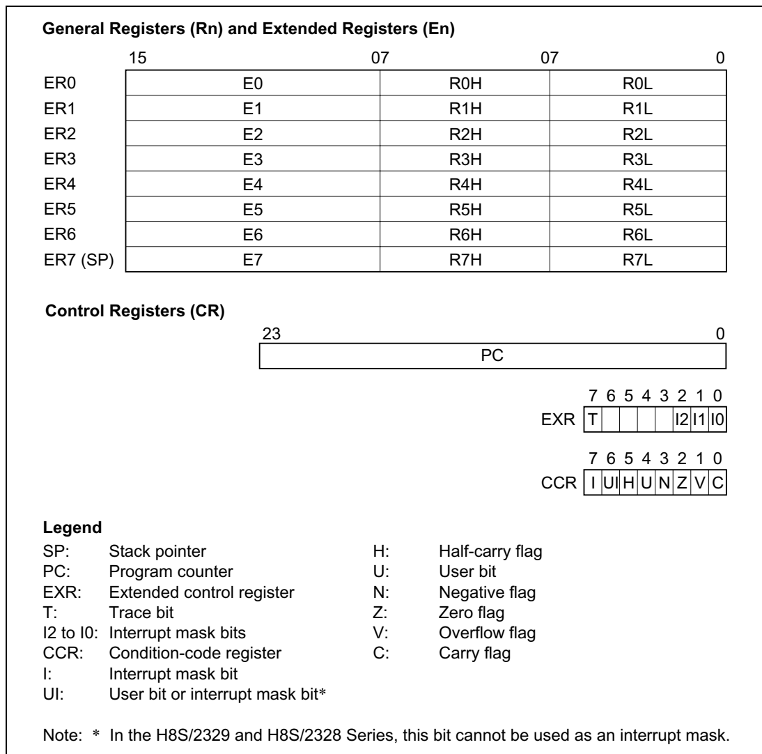
Figure 2-4 CPU Registers
