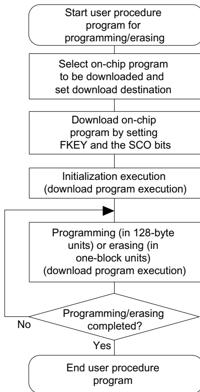
Figure 19-93 Overview of User Procedure Program
