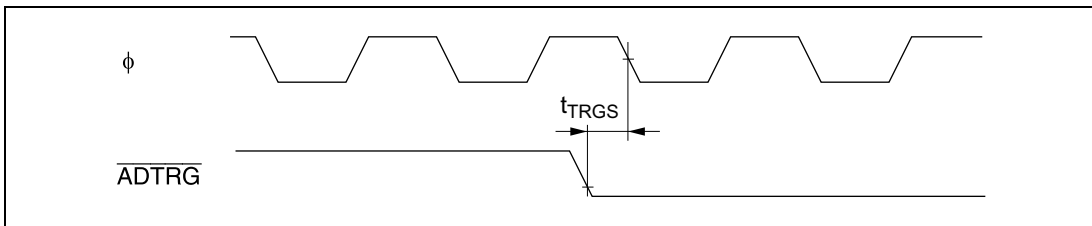
Figure 22-30 A/D Converter External Trigger Input Timing
