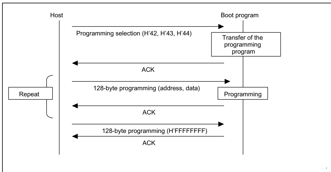
Figure 19-115 Programming Sequence
