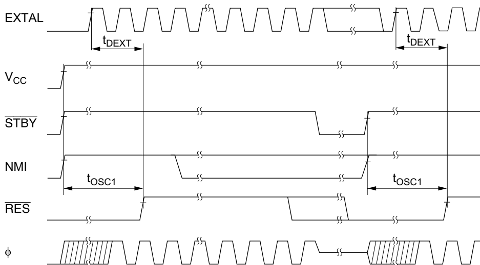
Figure 22-3 Oscillation Stabilization Timing
