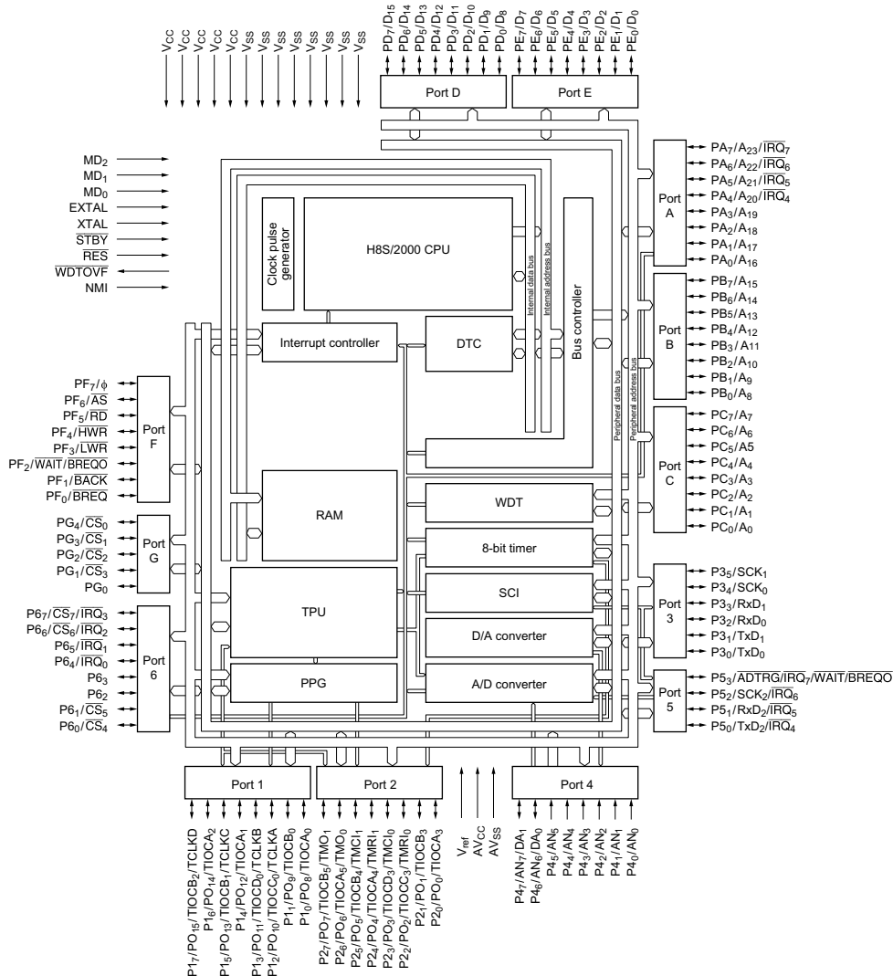
Figure 1-2 H8S/2321 Internal Block Diagram
