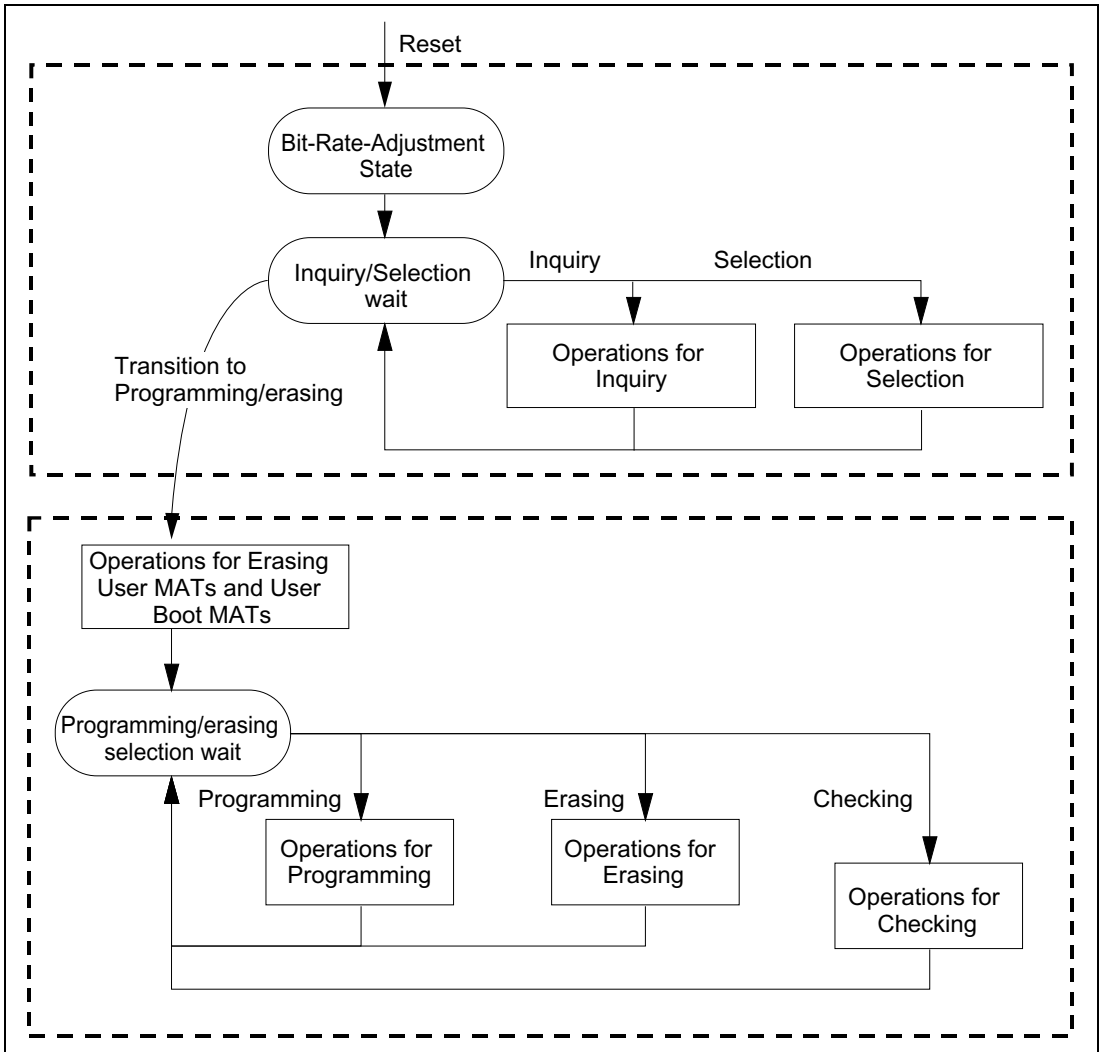
Figure 19-111 Boot Program States
