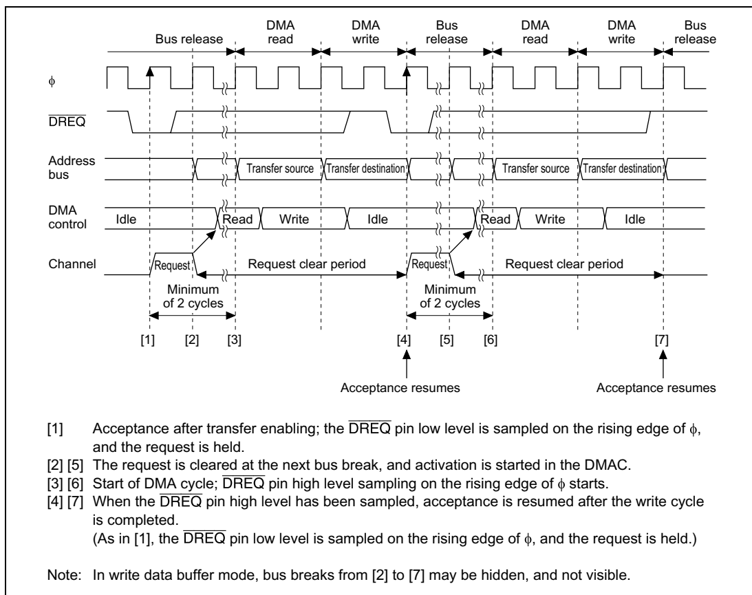
Figure 7-23 Example of DREQ Pin Falling Edge Activated Normal Mode Transfer
