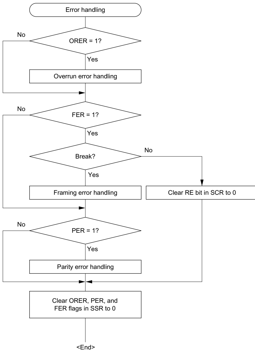
Figure 14-7 Sample Serial Reception Flowchart (cont)
