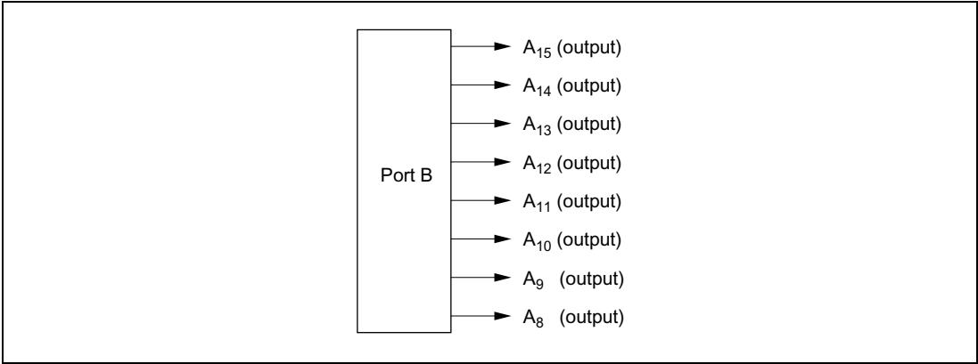
Figure 9-9 Port B Pin Functions (Modes 4 and 5)
