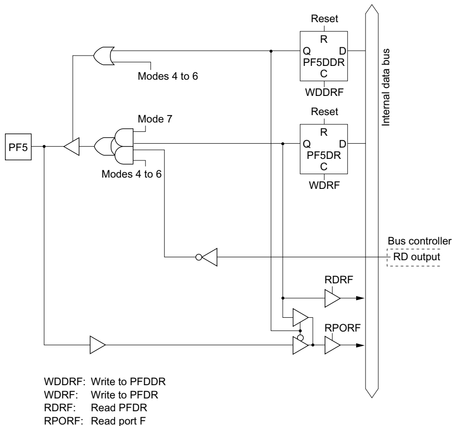
Figure C-12 (f) Port F Block Diagram (Pin PF 5 )
