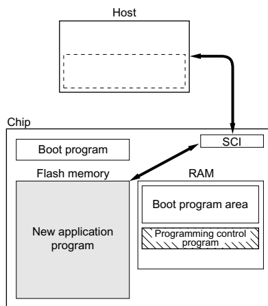
Figure 19-31 Boot Mode
