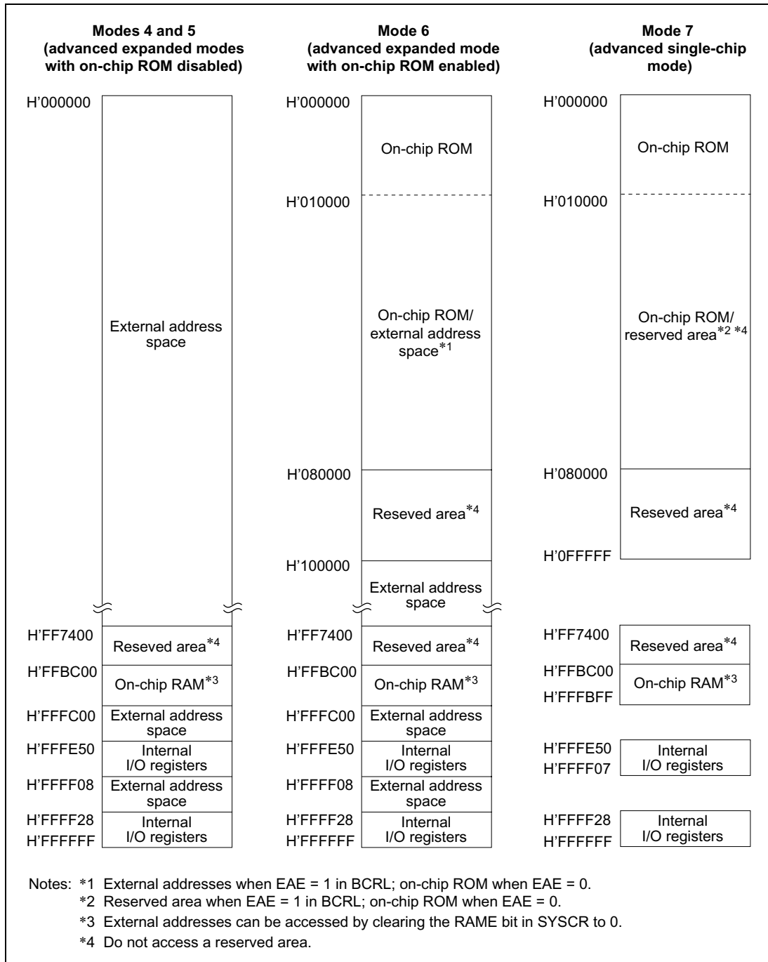
Figure 3-5(b) H8S/2326C F-ZTAT Address Map in Each Operating Mode
