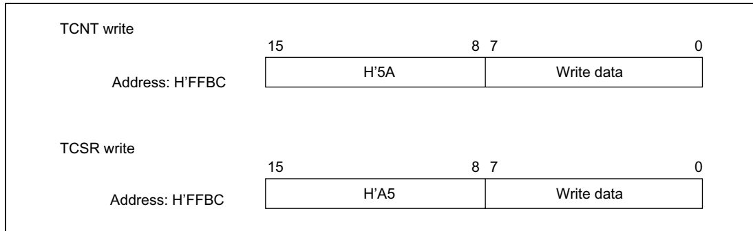
Figure 13-2 Writing to TCNT and TCSR
