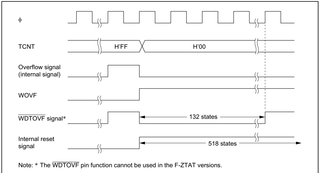
Figure 13-7 Timing of WOVF Setting
