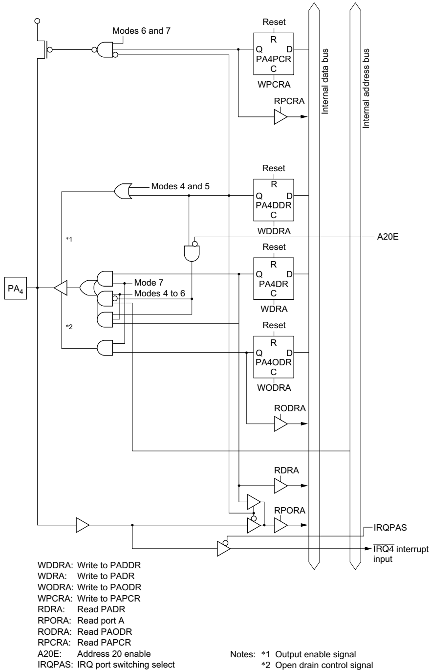
Figure C-7 (b) Port A Block Diagram (Pin PA 4 )
