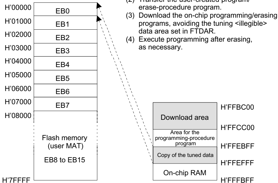
Figure 19-107 Programming of the Data After Tuning
