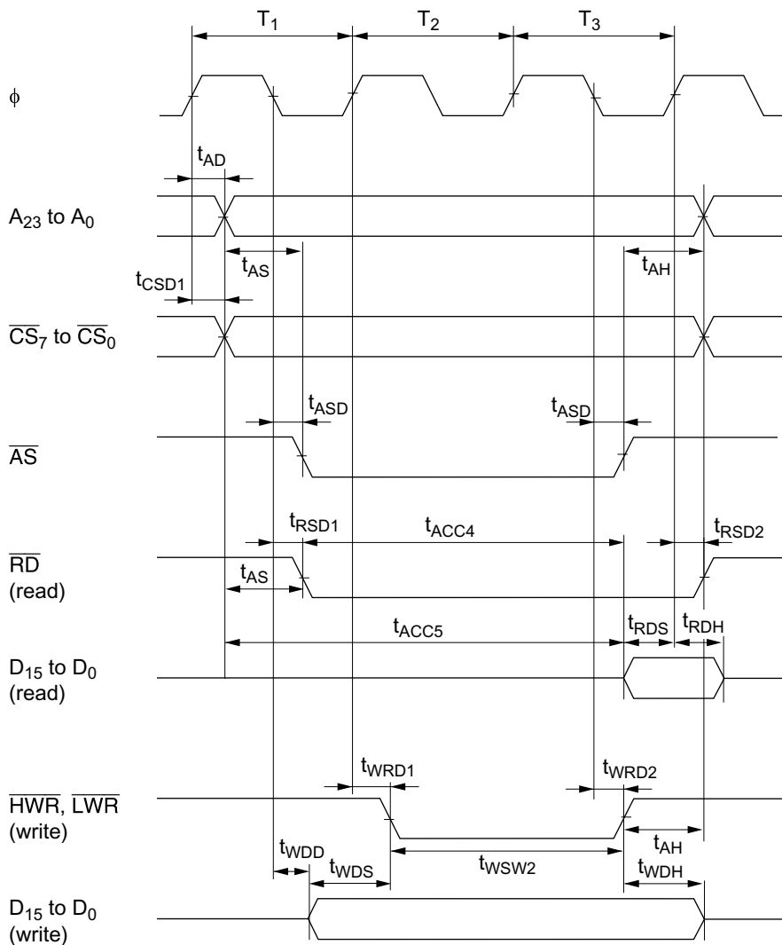
Figure 22-7 Basic Bus Timing (3-State Access)
