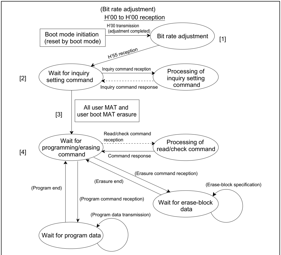
Figure 19-96 Overview of Boot Mode State Transition
