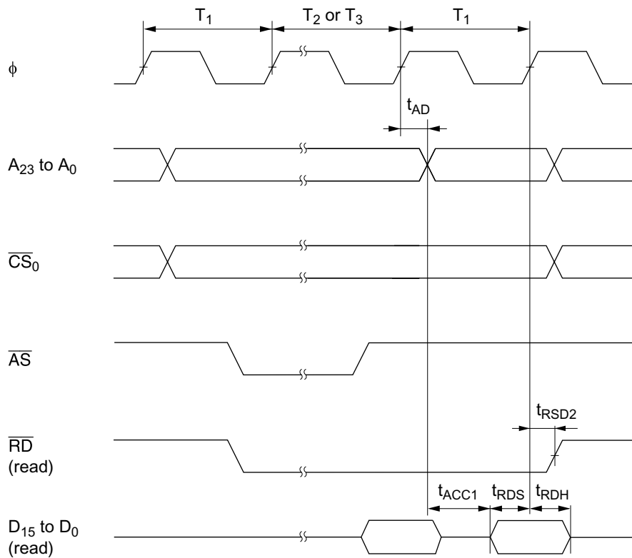
Figure 22-13 Burst ROM Access Timing (1-State Access)
