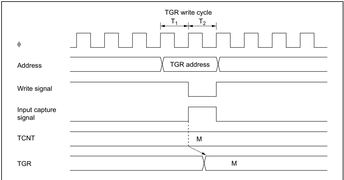
Figure 10-54 Contention between TGR Write and Input Capture
