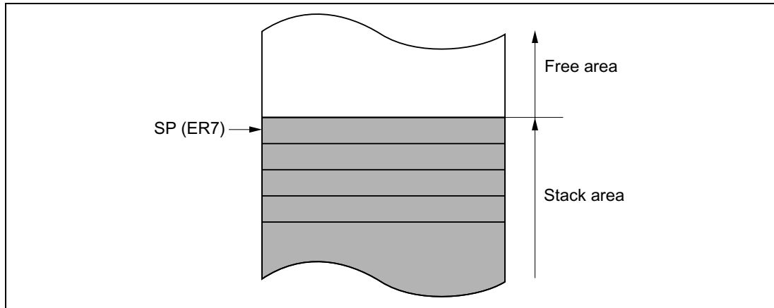
Figure 2-6 Stack
