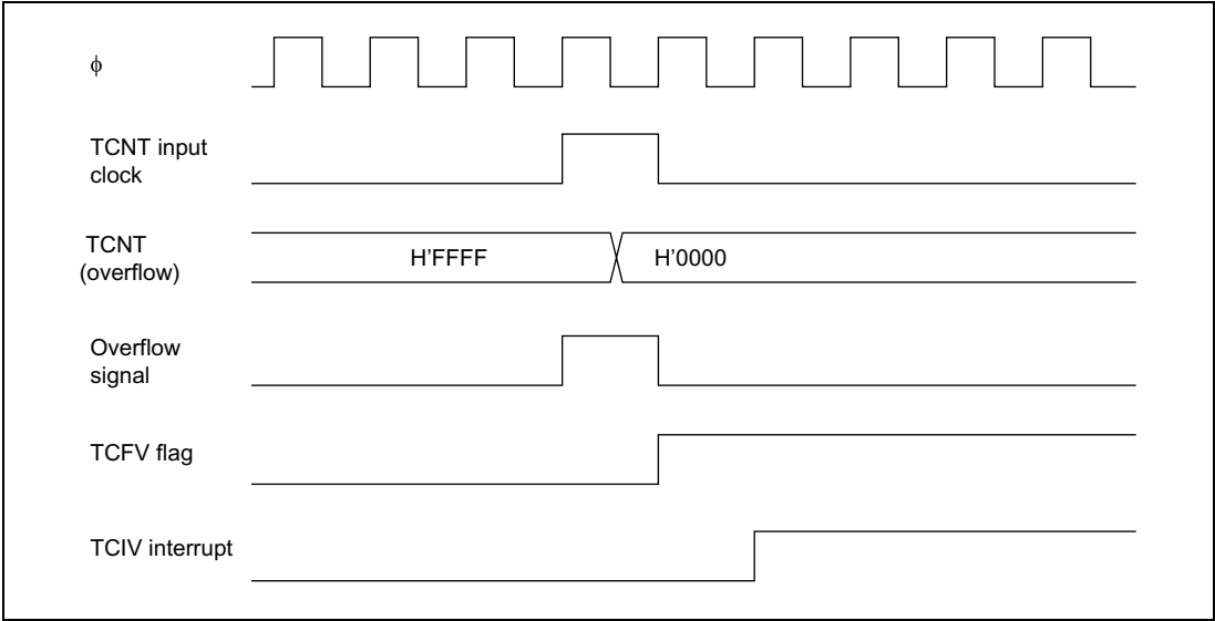
Figure 10-44 TCIV Interrupt Setting Timing
