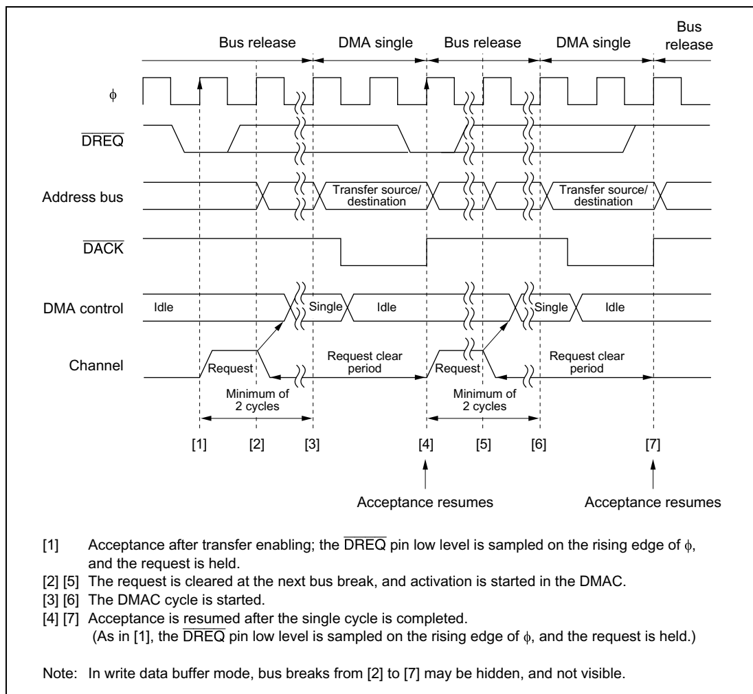
Figure 7-32 Example of DREQ Pin Low Level Activated Single Address Mode Transfer
