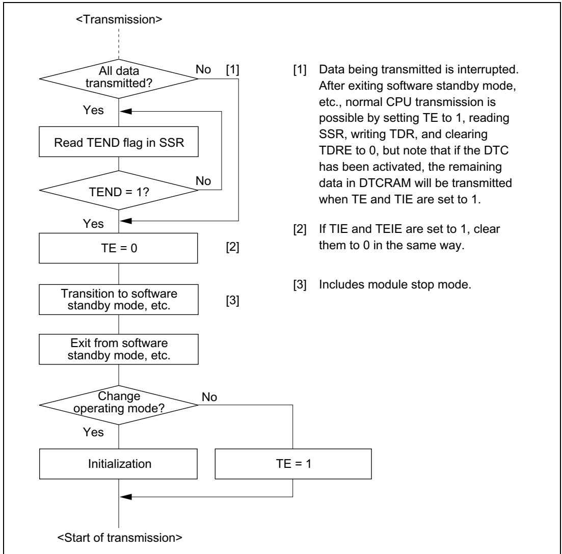
Figure 14-23 Sample Flowchart for Mode Transition during Transmission
