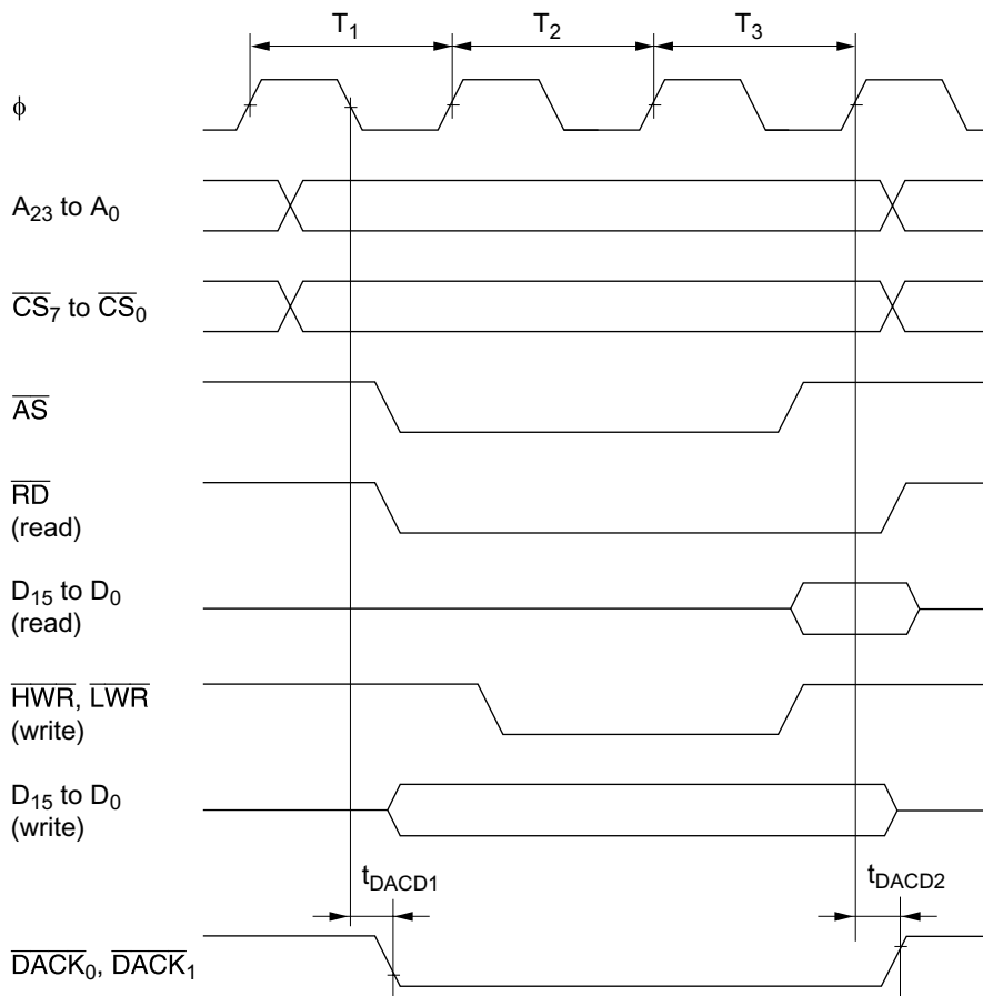
Figure 22-17 DMAC Single Address Transfer Timing (3-State Access)
