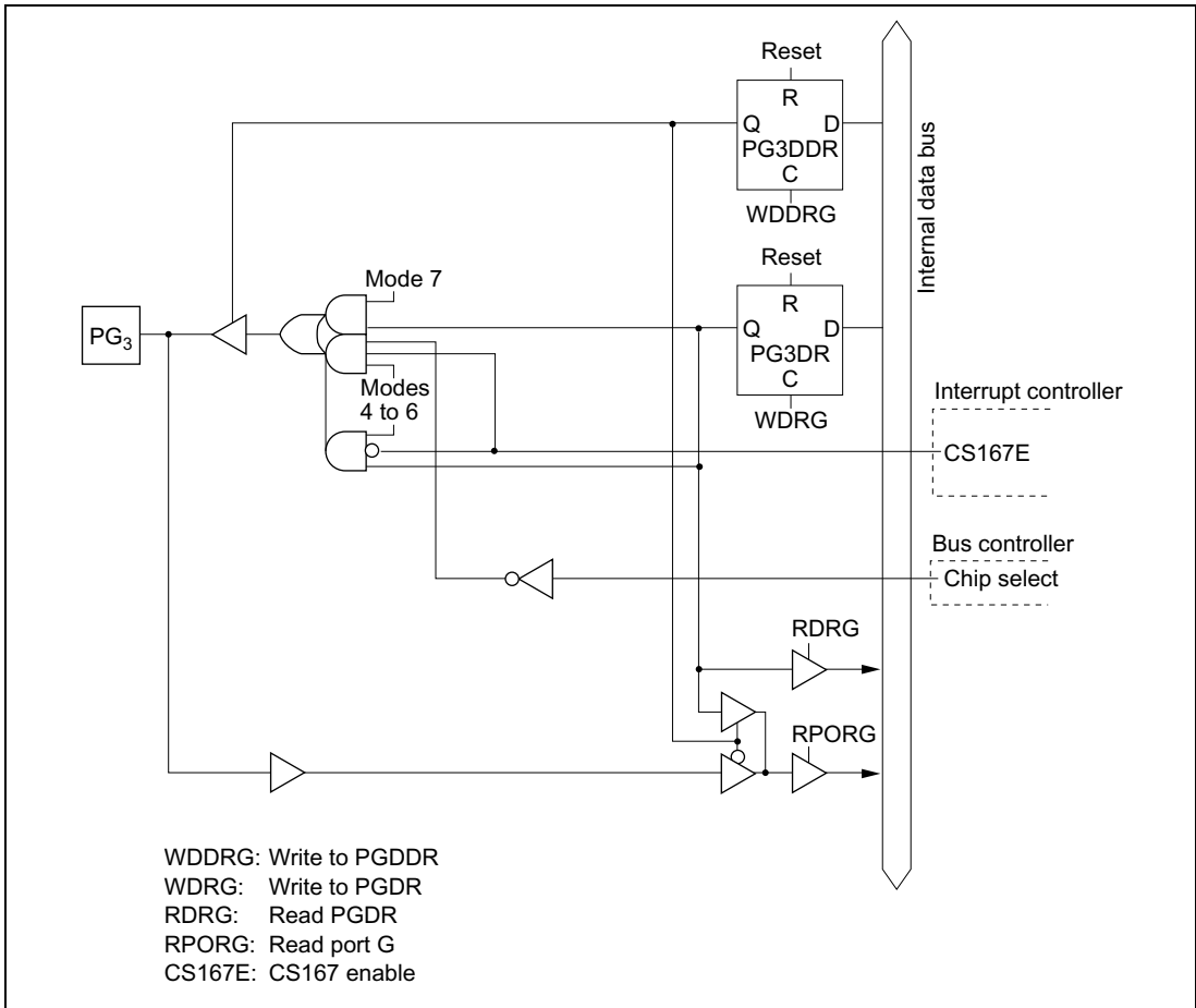
Figure C-13 (c) Port G Block Diagram (Pin PG 3 )
