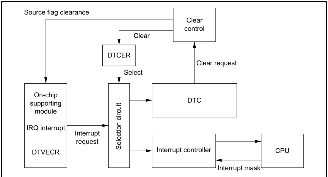
Figure 8-3 Block Diagram of DTC Activation Source Control
