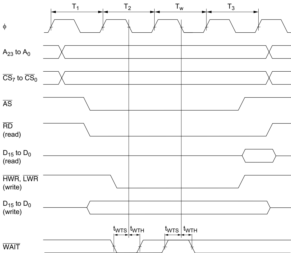
Figure 22-8 Basic Bus Timing (3-State Access, 1 Wait)
