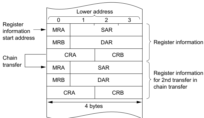
Figure 8-5 Location of DTC Register Information in Address Space
