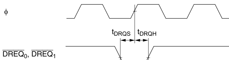
Figure 22-19 DMAC \overline{DREQ} Input Timing
