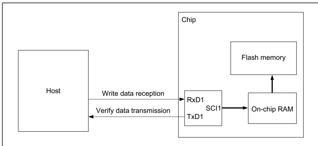
Figure 19-36 System Configuration in Boot Mode
