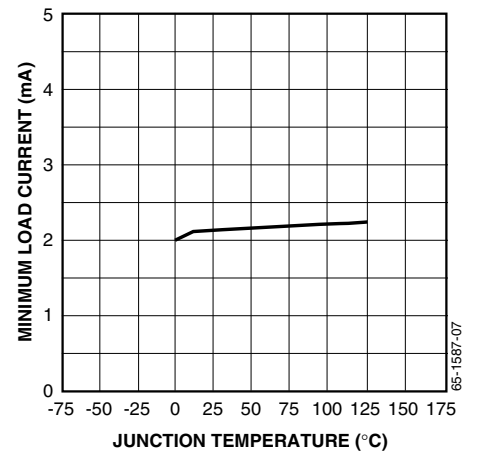
Figure 6. Minimum Load Current vs. Temperature
