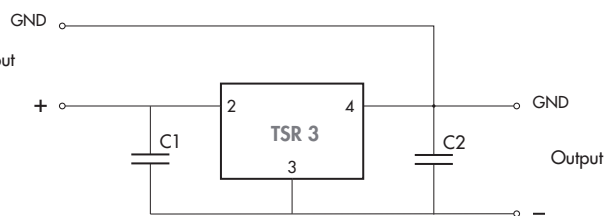
fig. 2 Negative output circuit
