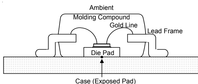
Figure 6. SOP-8 (Exposed Pad) Package Sectional Drawing
