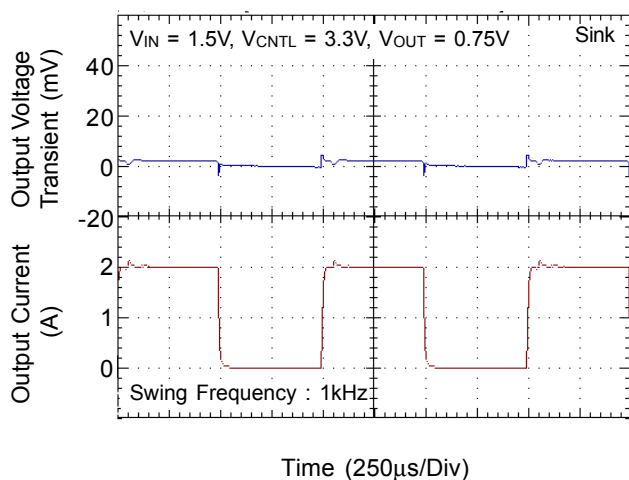
0.75V TT @ 2A Transient Response
