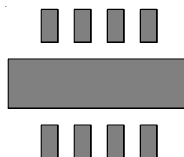
Figure 10 (c). Copper Area = 30mm 2 , \theta_{JA} = 54°C/W
