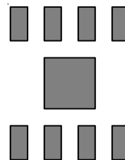
Figure 10 (a). Minimum Footprint, \theta_{JA} = 75°C/W
