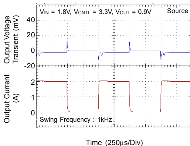
0.9V TT @ 2A Transient Response
