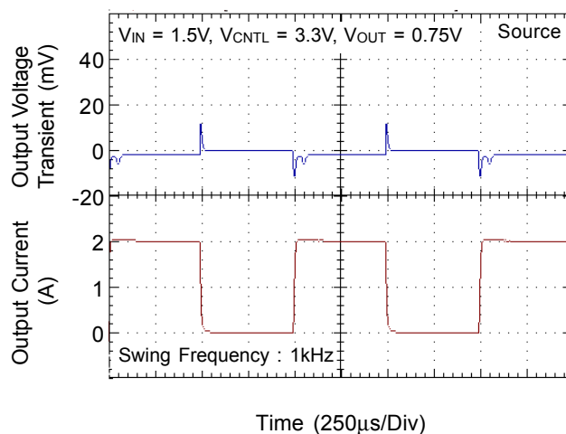
0.75V TT @ 2A Transient Response
