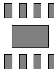
Figure 10 (b). Copper Area = 10mm 2 , \theta_{JA} = 64°C/W
