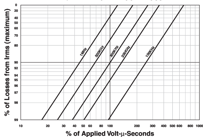
I IRMS DERATING WITH CORE LOSS
