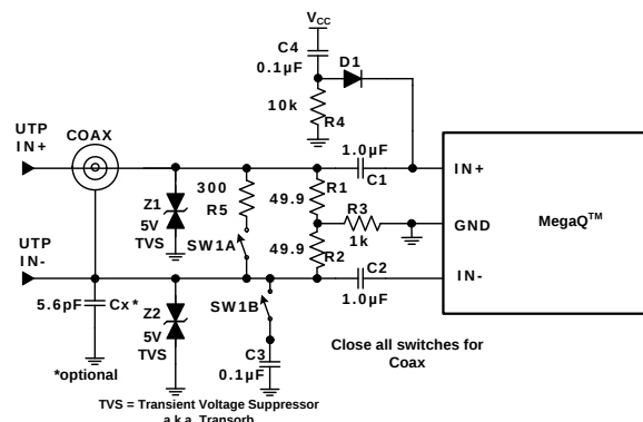
FIGURE 47. APPLICATION CIRCUIT FOR UTP/COAX CABLE
