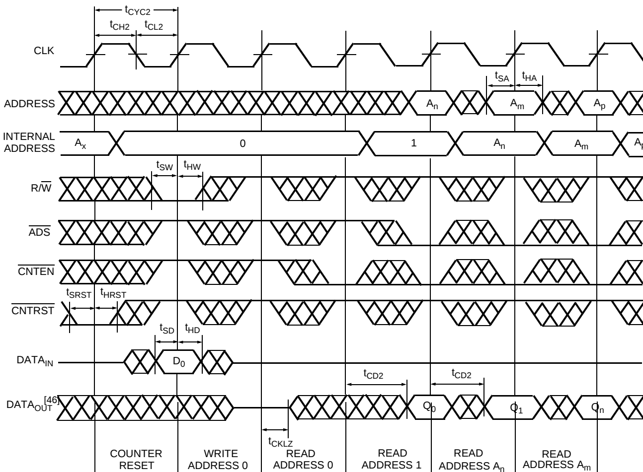
Figure 19. Counter Reset [44, 45, 46]
