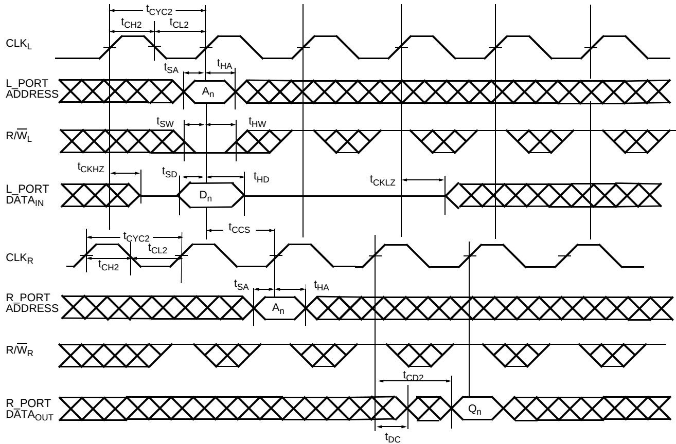
Figure 21. Left_Port (L_Port) Write to Right_Port (R_Port) Read [51, 52, 53]
