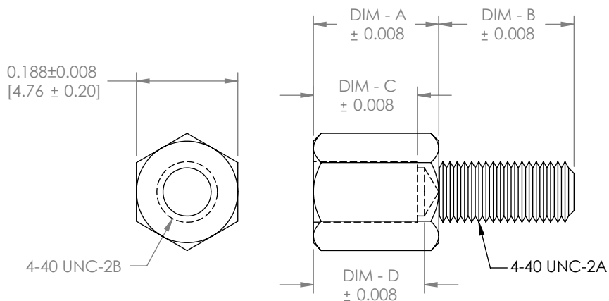
JACK-SCREW
