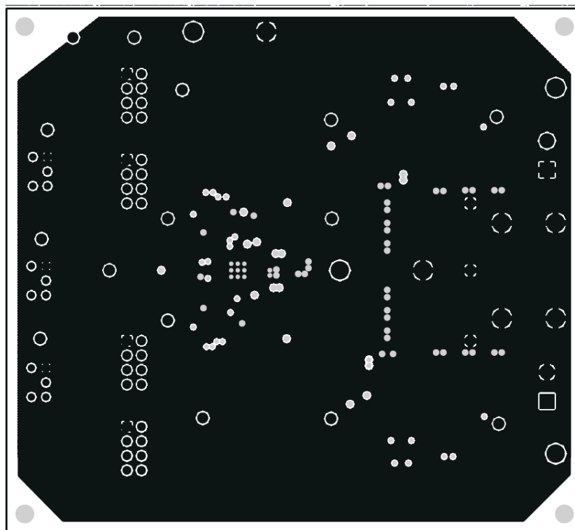
Figure 7-2. Inner Layer 1
