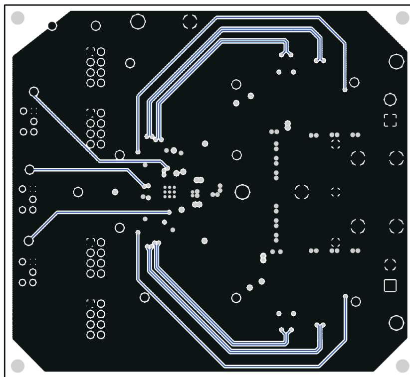
Figure 7-3. Inner Layer 2
