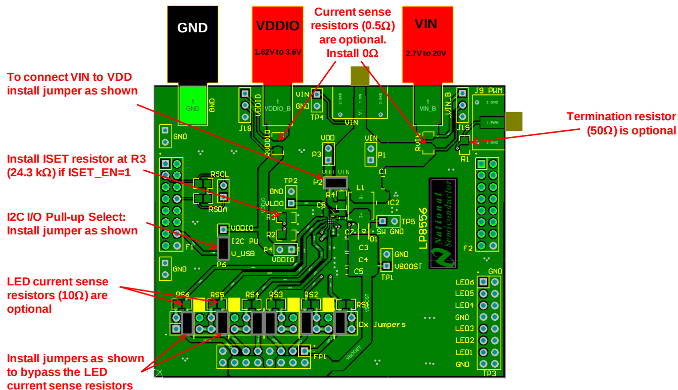
Figure 3: LP8556TM-EVM Configuration
