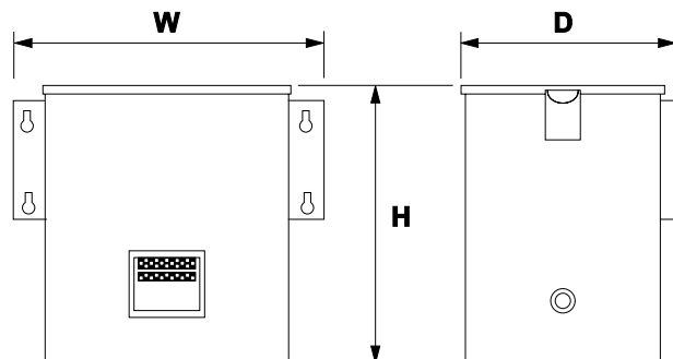
Style 4 - Encapsulated
