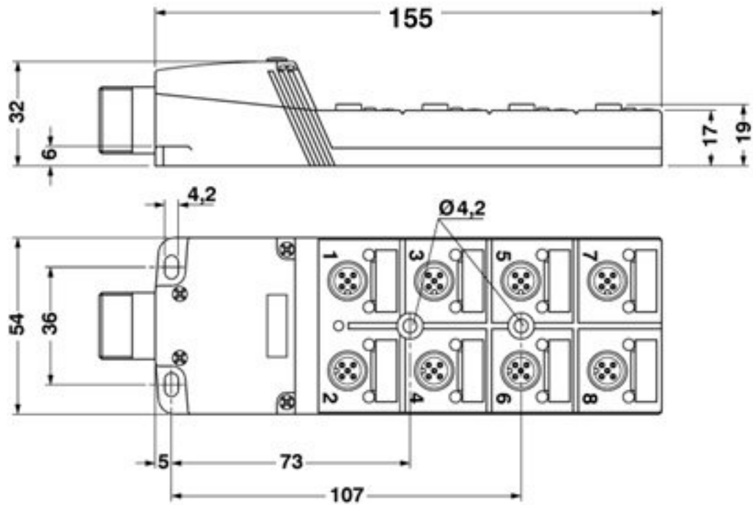
Dimensioned drawing
