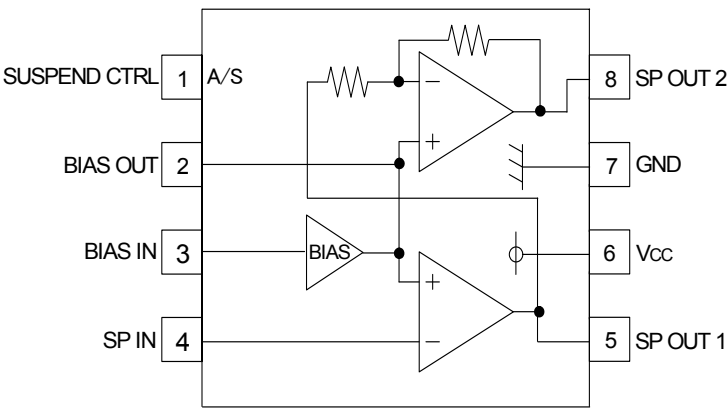
Fig.4 BH7824FVM
