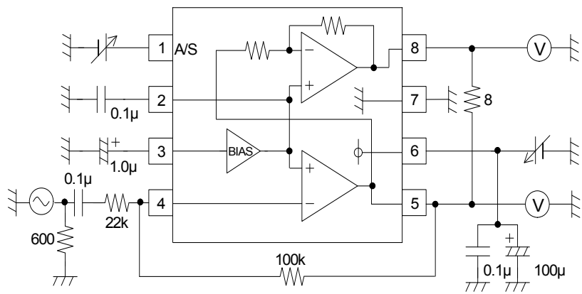
Fig.2 BH7824FVM
