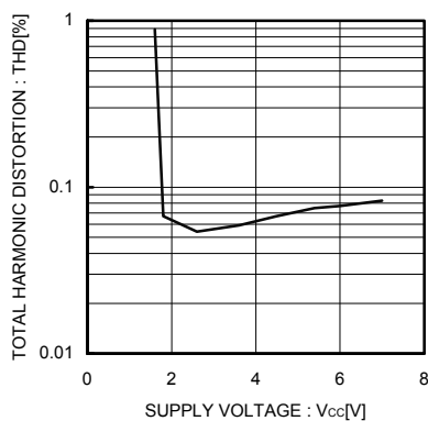
Fig.12 Total harmonic distortion vs Supply voltage
