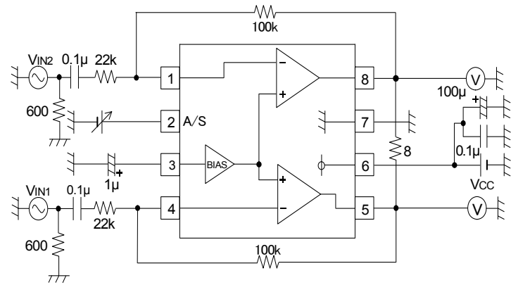
Fig.3 BH7826FVM
