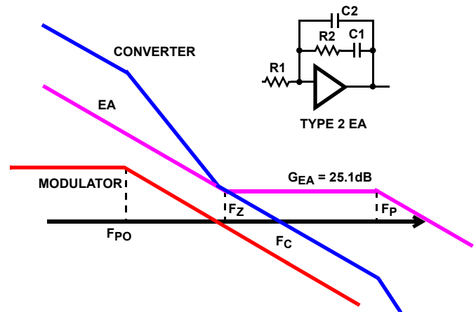
FIGURE 27. FEEDBACK LOOP COMPENSATION
