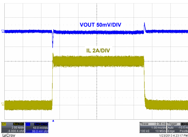
FIGURE 16. LOAD TRANSIENT 100%
