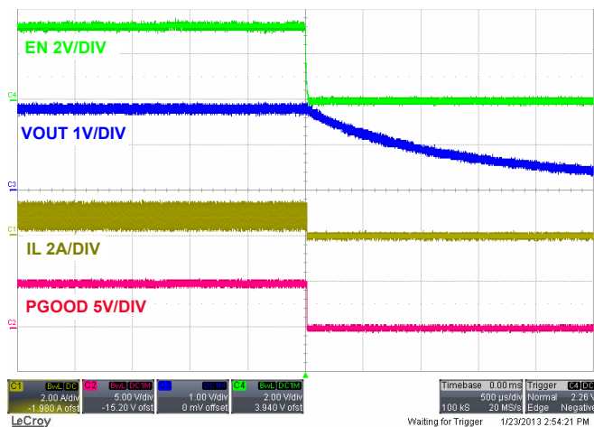
FIGURE 18. SOFT-DISCHARGE SHUTDOWN
