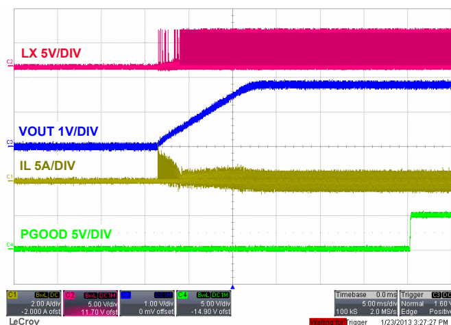
FIGURE 20. OUTPUT SHORT CIRCUIT RECOVERY
