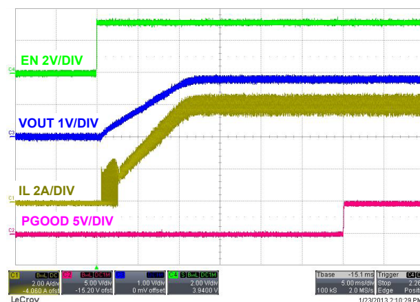
FIGURE 12. SOFT-START WITH FULL LOAD
