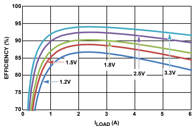
FIGURE 6. EFFICIENCY vs LOAD, V_{IN} = 5.0\text{V}
