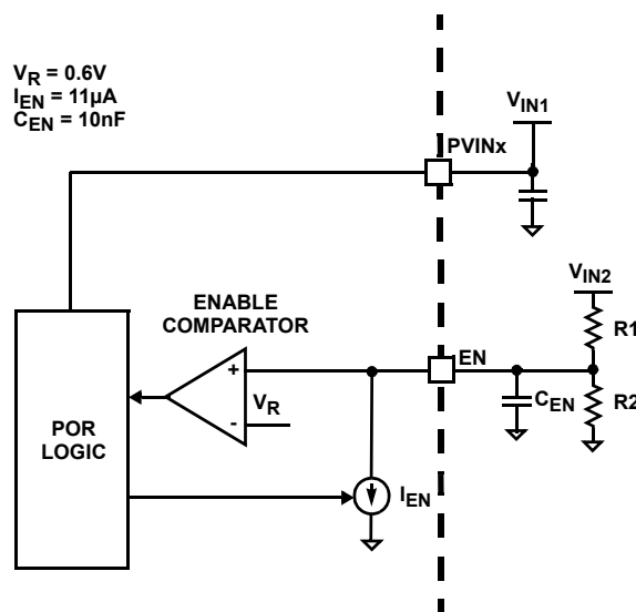
FIGURE 24. ENABLE CIRCUIT
