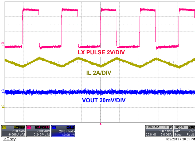
FIGURE 14. STEADY STATE OPERATION WITH FULL LOAD
