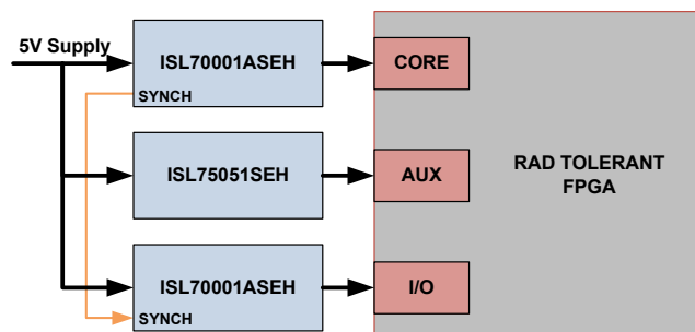
FIGURE 1. TYPICAL APPLICATION
