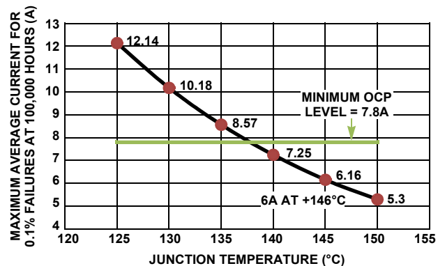
FIGURE 28. CURRENT vs TEMPERATURE
