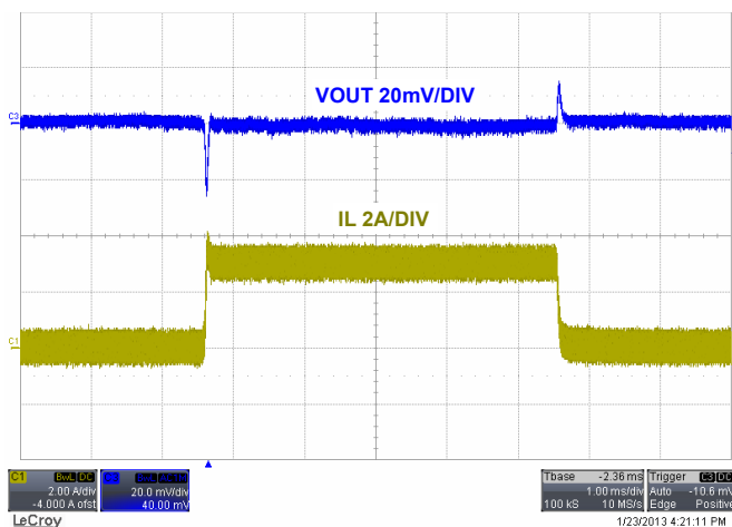
FIGURE 15. LOAD TRANSIENT 50%
