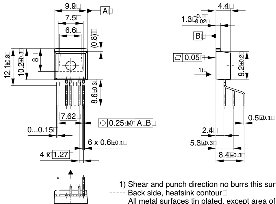
Figure 60 PG-TO220-6-46 (Isodrain Package)
