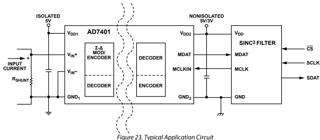
Figure 23. Typical Application Circuit
