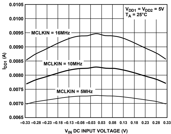
Figure 14. I_{DD1} vs. V_{IN}
