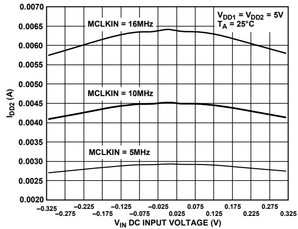
Figure 16. I_{DD2} vs. V_{IN}
