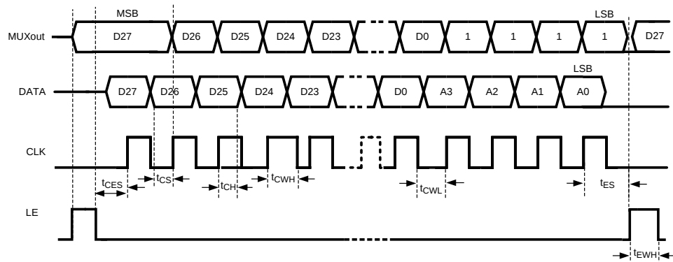
Figure 18. Timing for Readback
