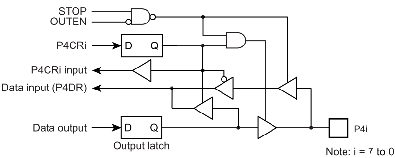
Figure 5-6 Port P4
