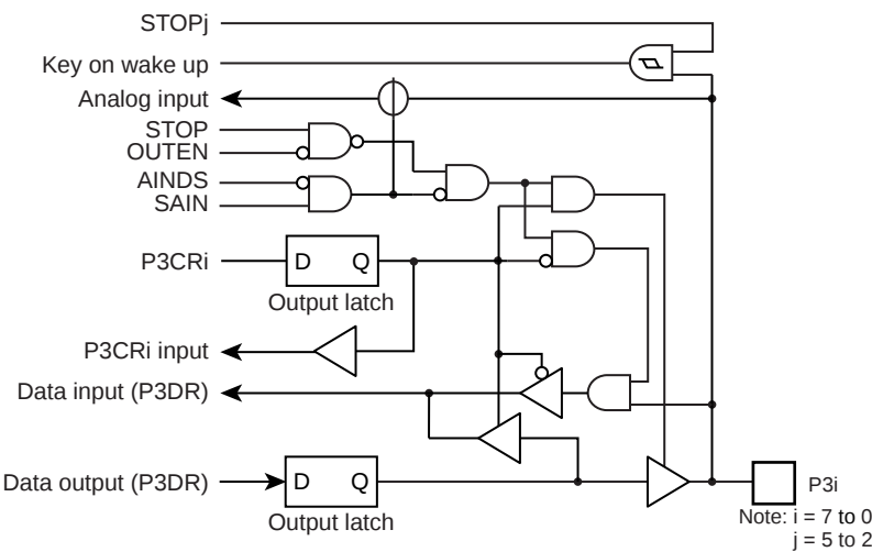
Figure 5-5 Port P3
