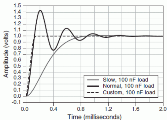
1 mA Range, 100 nF Load Step Response, typical
