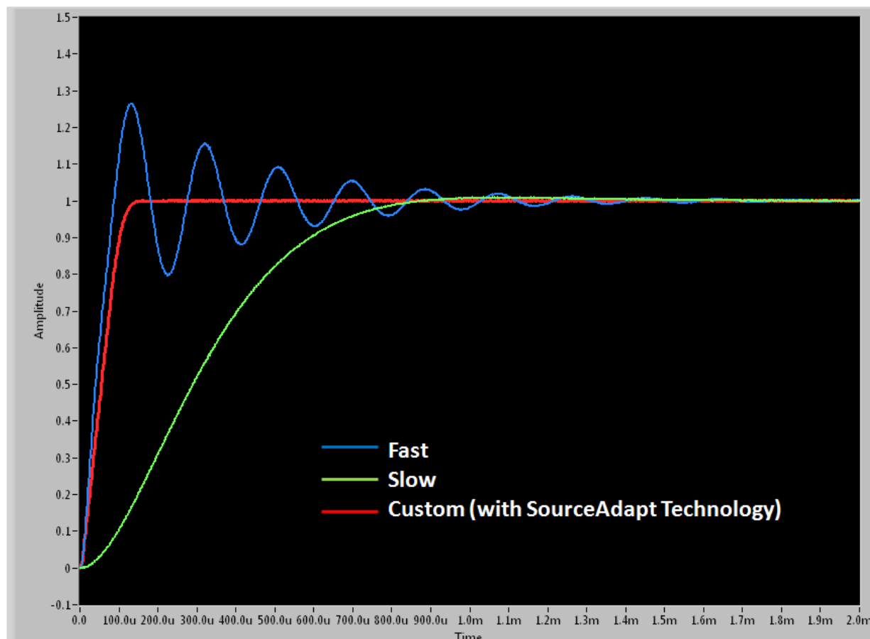
Figure 1. SMU Response to a Capacitive Load
