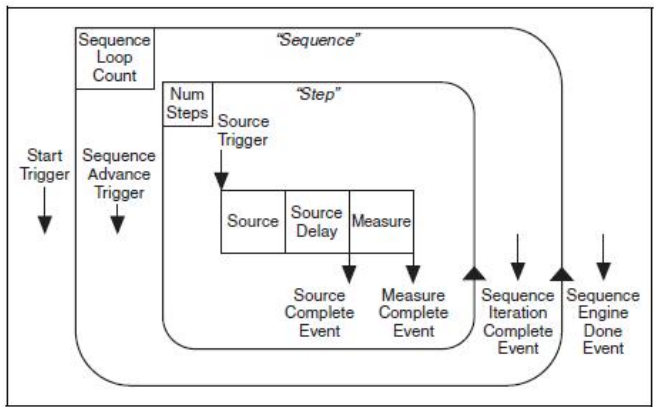
Figure 5. NI-DCPower Programming Flow
