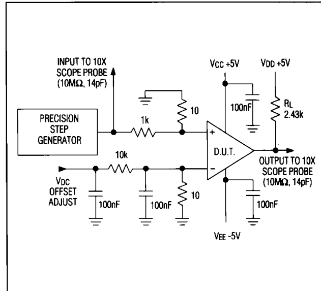
Figure 5. Response-Time Setup
