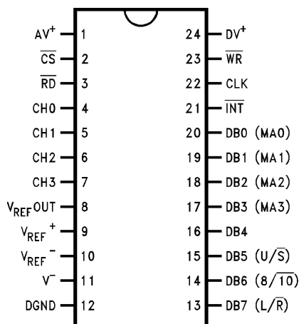
Dual-in-Line and SO Packages
