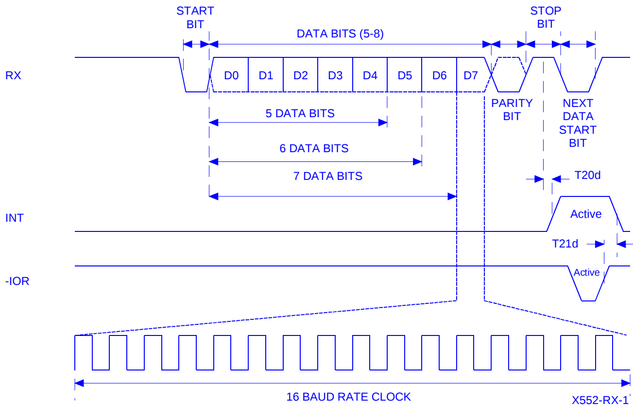
Receive timing
