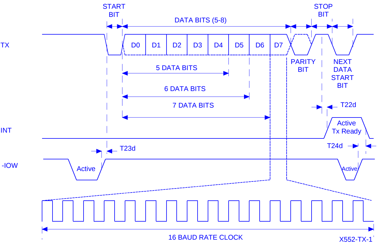
Transmit timing
