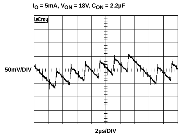
FIGURE 16. V_{ON} RIPPLE
