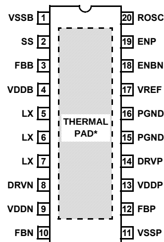
EL7581 (20 LD HTSSOP) TOP VIEW
