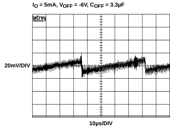
FIGURE 18. V_{OFF} RIPPLE
