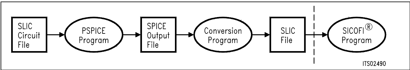
Figure 3 Software Structure
