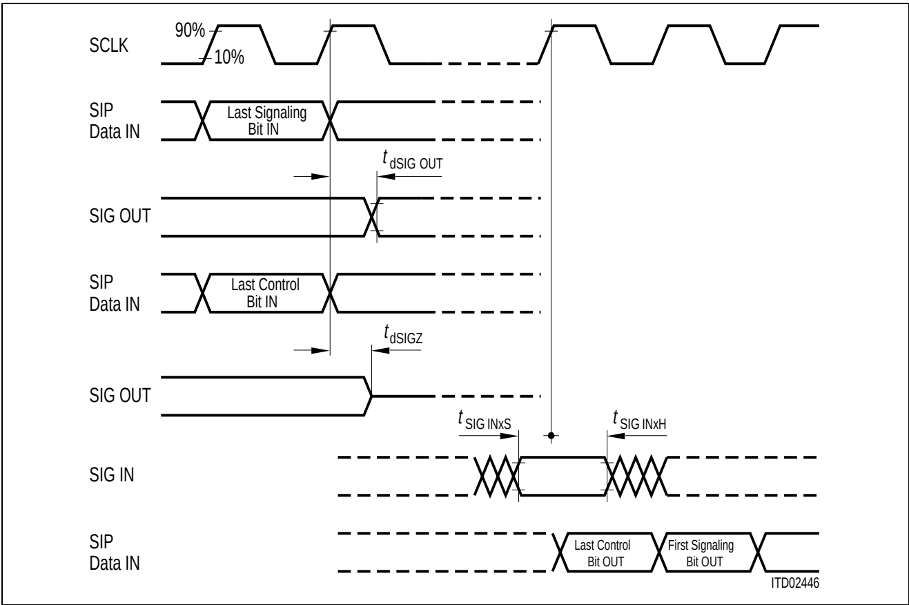
Signaling Interface Timing (SLD)
