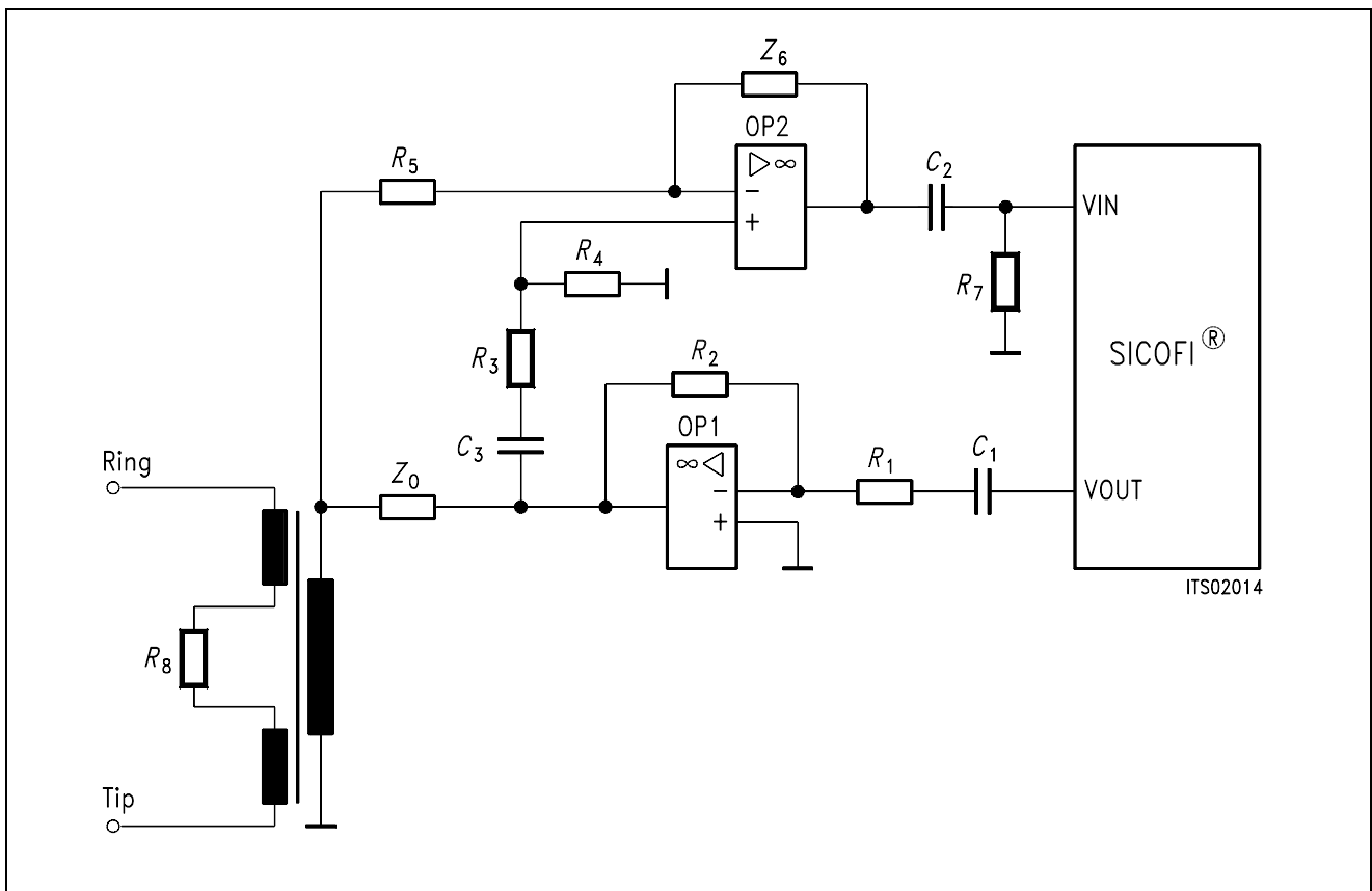
Figure 12 SLIC Circuit
