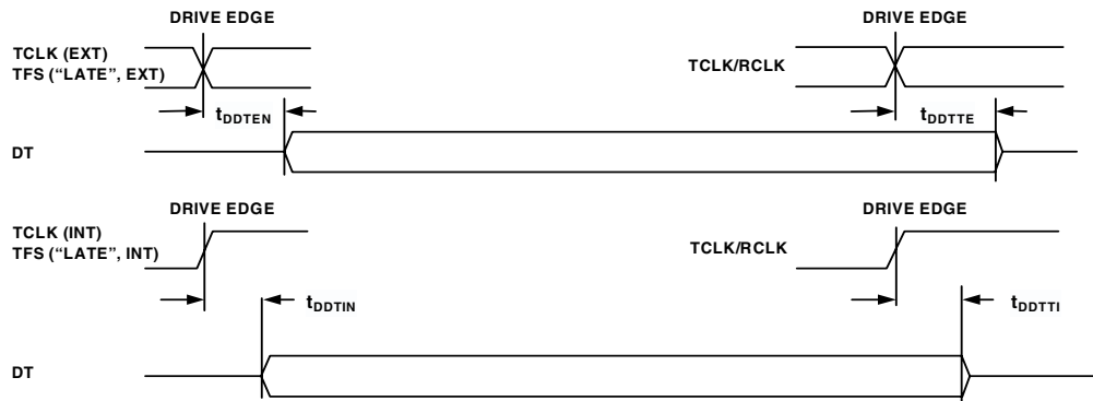
Figure 13. Serial Ports
