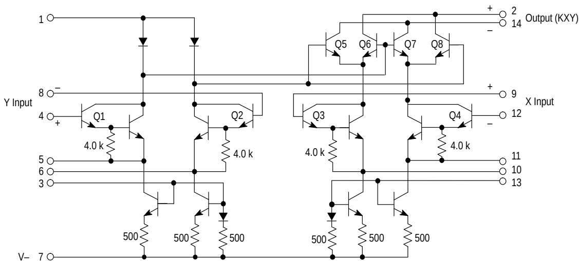
Figure 3. Circuit Schematic
