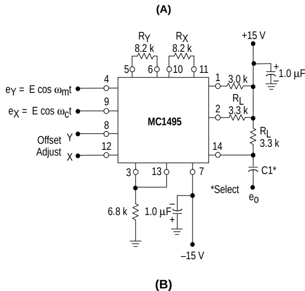
Figure 29. Balanced Modulator
