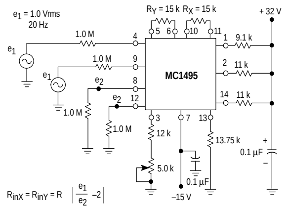
Figure 7. Input Resistance
