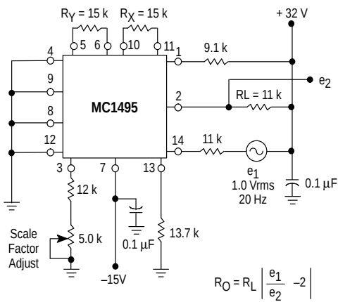
Figure 8. Output Resistance
