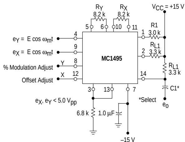
Figure 30. Amplitude Modulation
