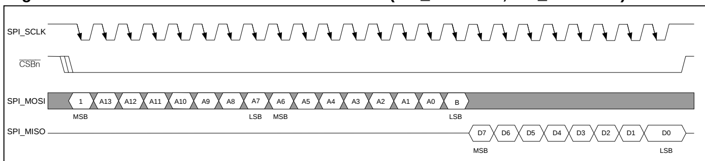
Figure 8-3. SPI Serial Port Access for Read Mode (SPI_CPOL = 0, SPI_CPHA = 1)
