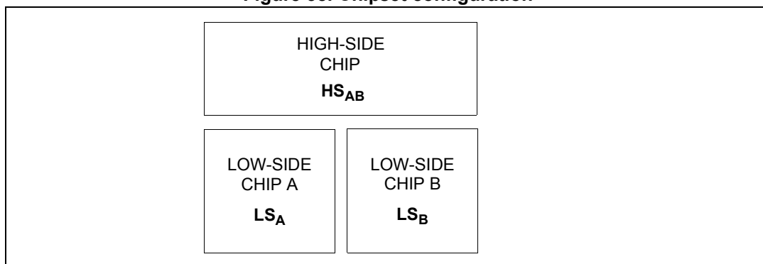
Figure 38. Chipset configuration
