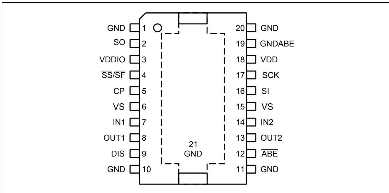
Figure 1 Pinout TLE8209-2SA
