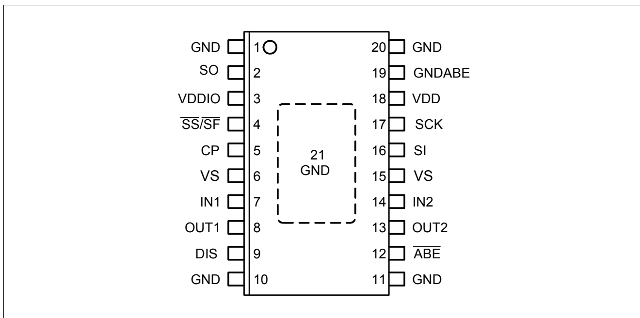
Figure 2 Pinout TLE8209-2E
