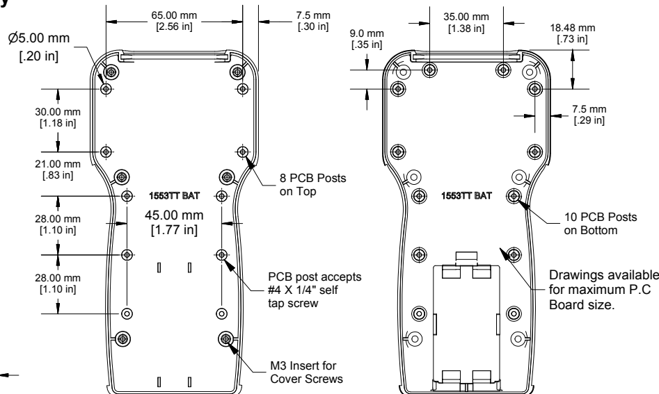
Inside View of Bottom
