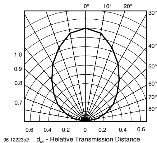
Fig. 12 - Horizontal Directivity
