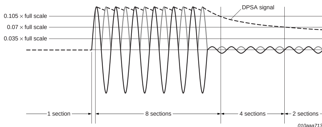
Fig 7. Dynamic Power Stage Activation
