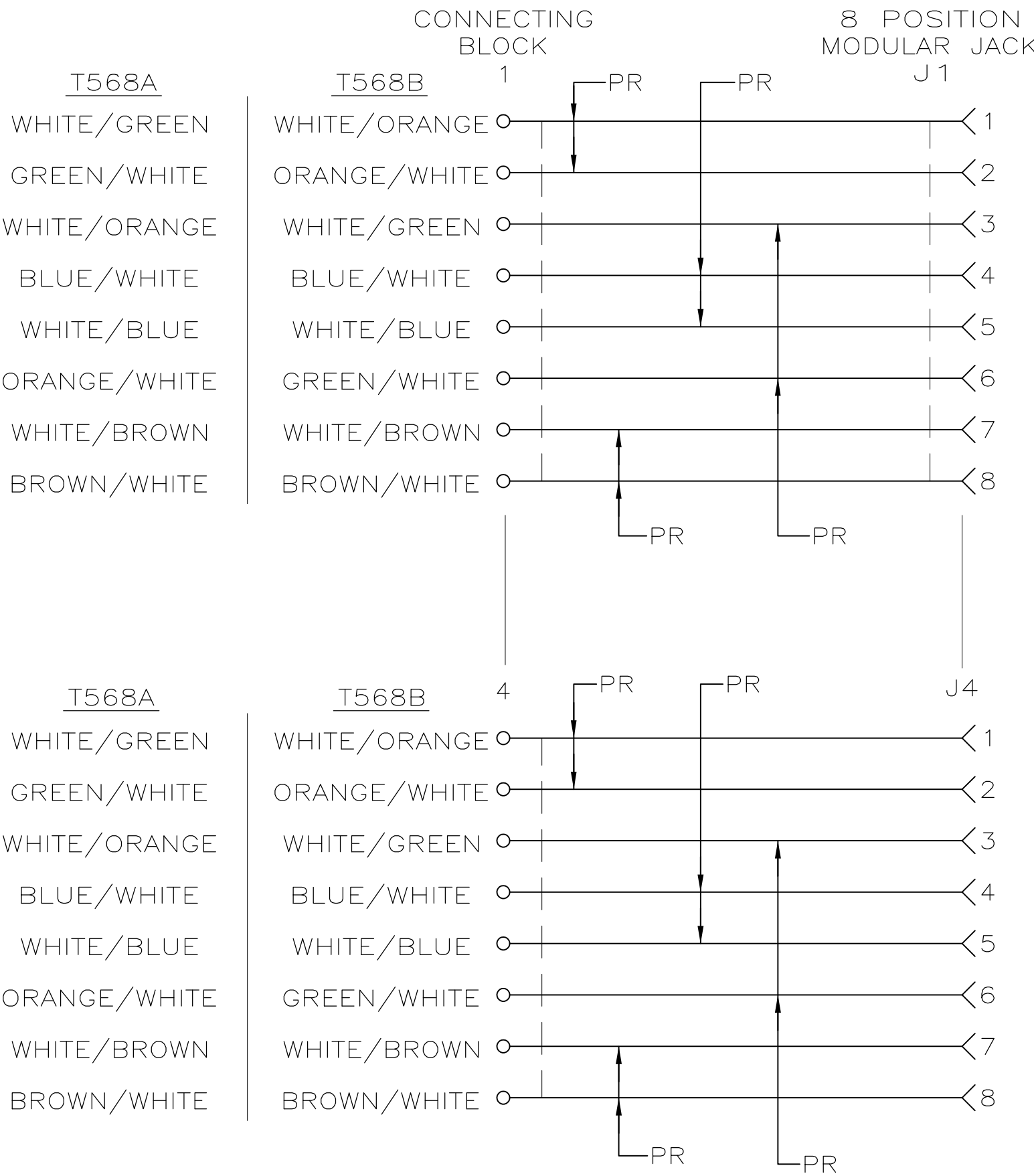
ELECTRICAL SCHEMATIC FOR T568A OR T568B WIRING PATTERN
