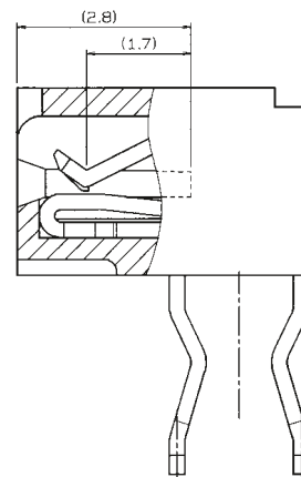
SECT W-W
