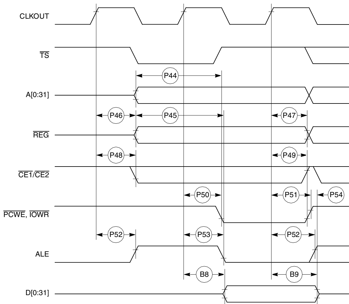
Figure 29. PCMCIA Access Cycles Timing External Bus Write
