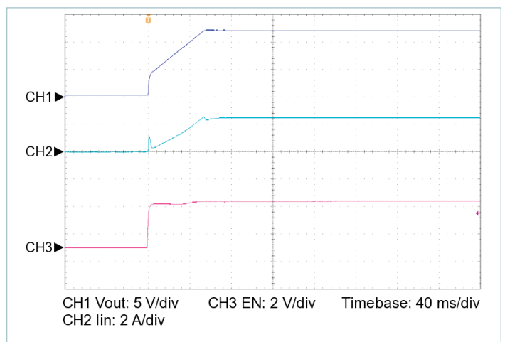
Figure 14 — Startup from EN, V_{IN} = 100\text{ V} , C_{OUT\_EXT} = 20000\text{ }\mu\text{F} , R_{LOAD} = 0.600\text{ }\Omega
