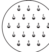
24-19 19#12 (I)
