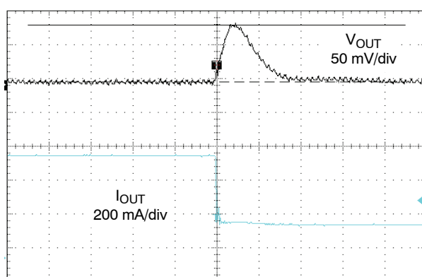
Figure 26. 200 mA to 100 mA Load Transient ( V_{IN} = 3.6\text{ V} , V_{OUT} = 1.2\text{ V} , T_A = 25^\circ\text{C} )
