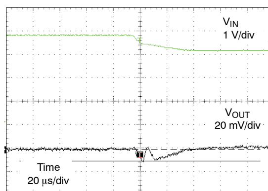
Figure 20. 3.6 V to 3.0 V Line Transient (Risetime = 50\text{ μs} , V_{OUT} = 1.2\text{ V} , I_{OUT} = 100\text{ mA} , T_A = 25^\circ\text{C} )
