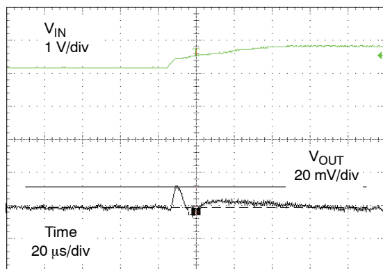
Figure 19. 3.0 V to 3.6 V Line Transient (Risetime = 50\text{ μs} , V_{OUT} = 1.2\text{ V} , I_{OUT} = 100\text{ mA} , T_A = 25^\circ\text{C} )
