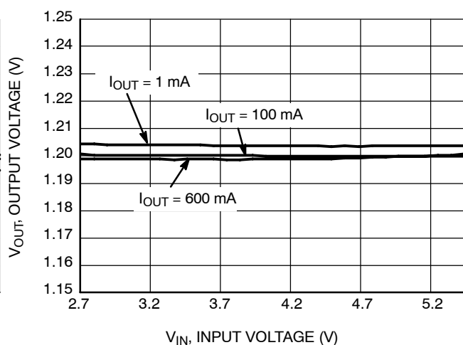
Figure 18. Line Regulation ( V_{OUT} = 3.6\text{ V} , T_A = 25^\circ\text{C} )
