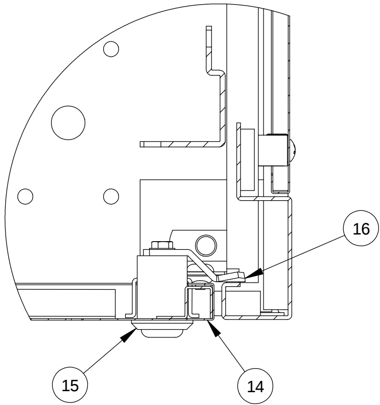
DETAIL D SCALE 1 : 2
