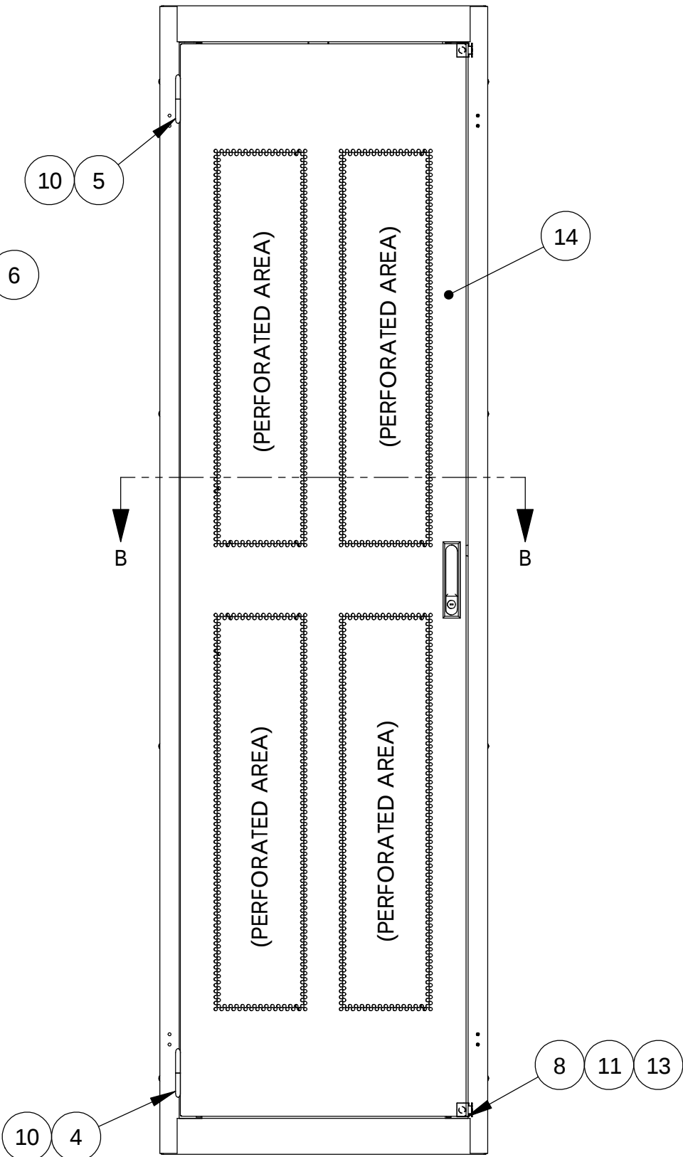
REAR VIEW
