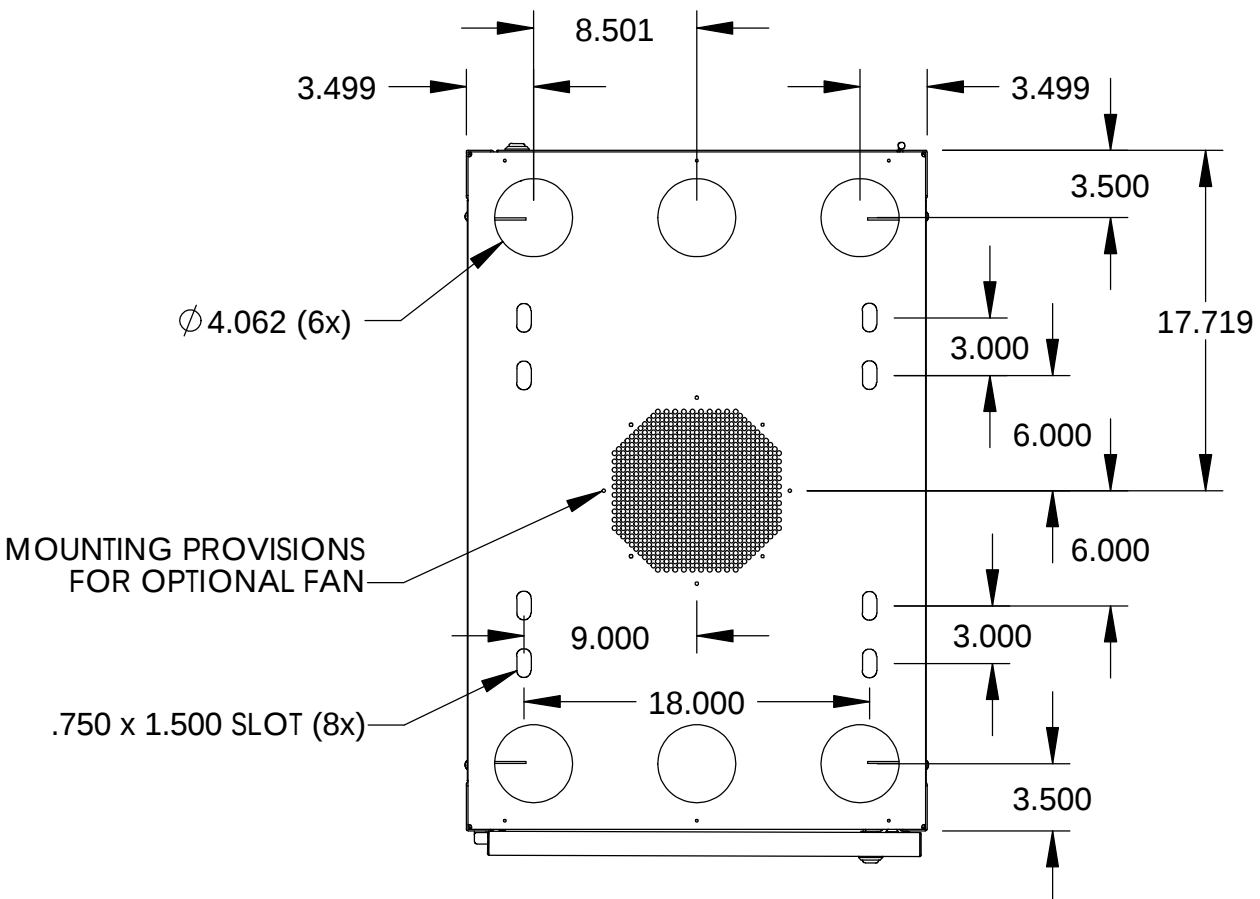
TOP VIEW
