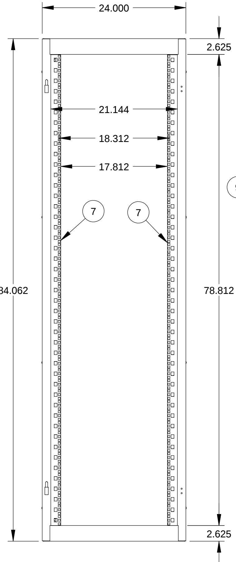
FRONT VIEW (LESS DOOR)
