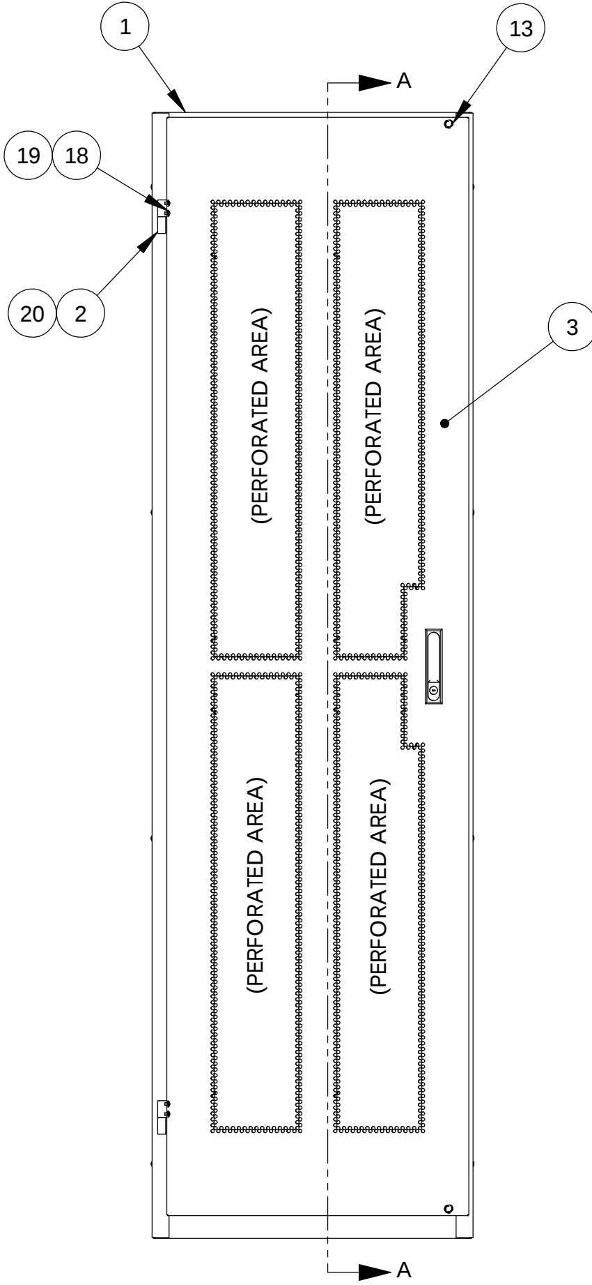
FRONT VIEW
