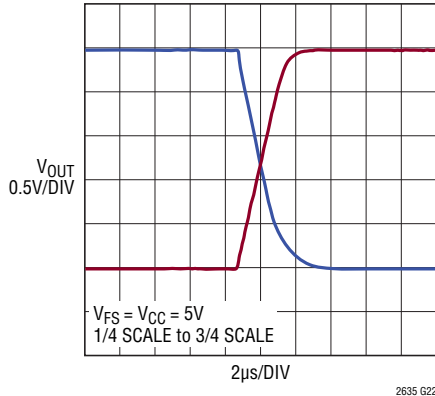
Large-Signal Response
