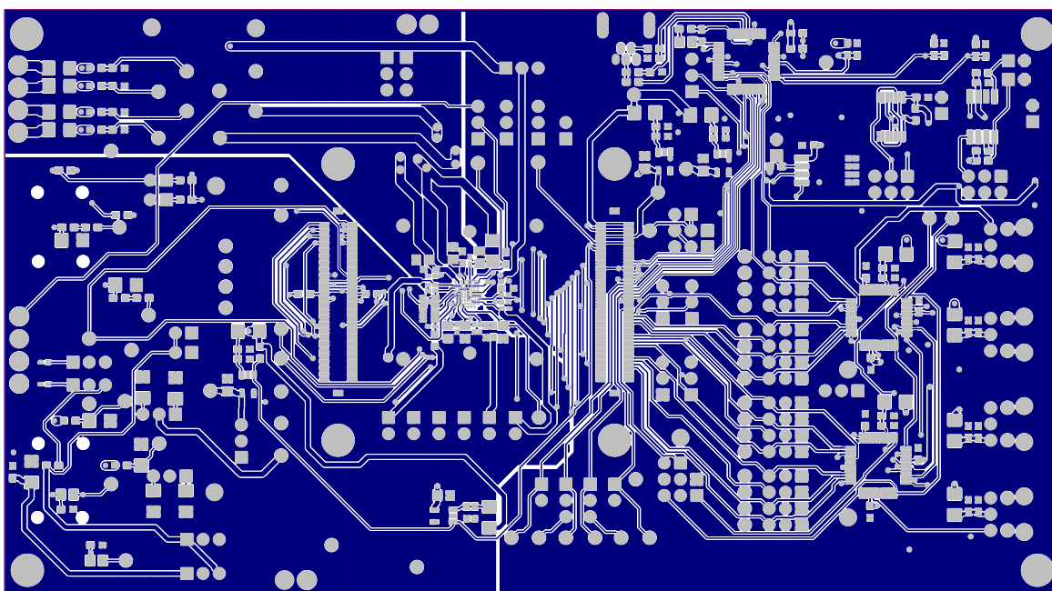
Figure 12. TLV320AIC3212EVM PCB Bottom Copper, Reversed
