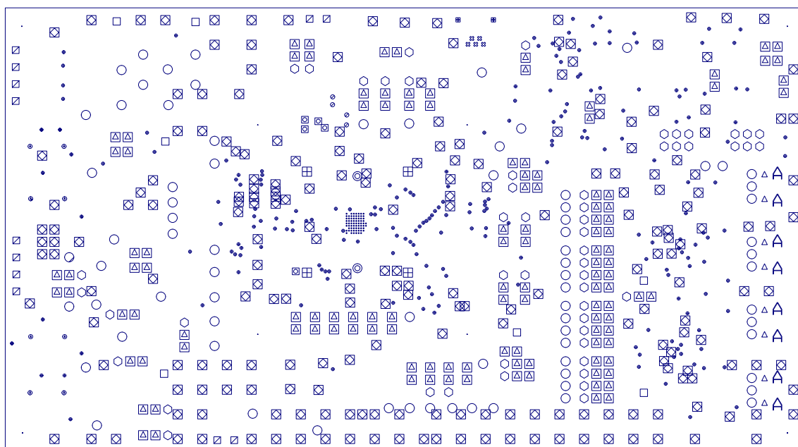
Figure 14. TLV320AIC3212EVM PCB Drill Pattern
