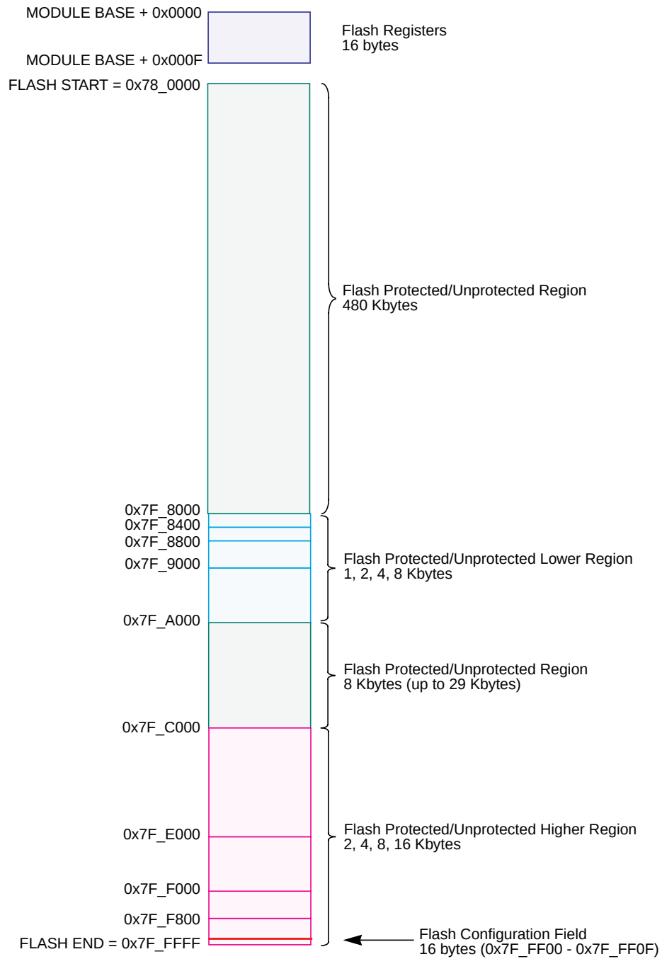
Figure 3-2. Flash Memory Map
