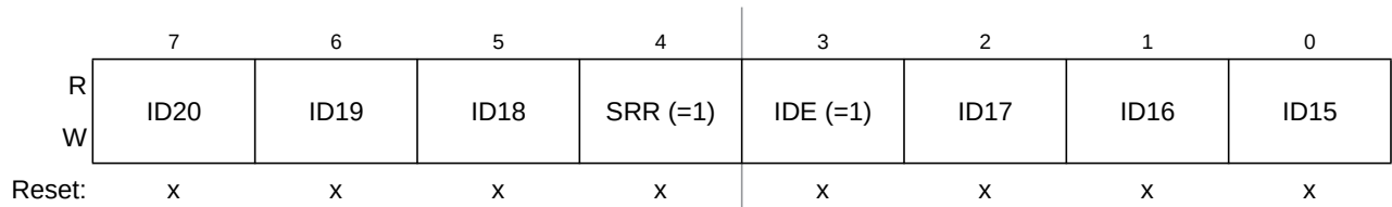
Figure 14-27. Identifier Register 1 (IDR1) — Extended Identifier Mapping
