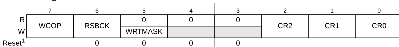
Figure 7-12. CRG COP Control Register (COPCTL)
