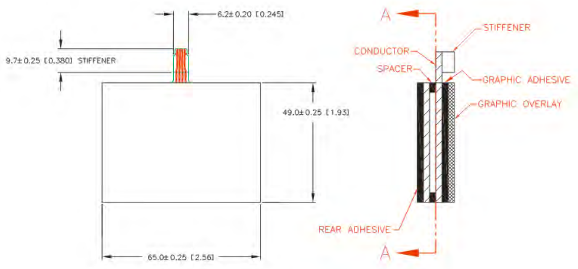
Figure 9: VersaPad Sensor
