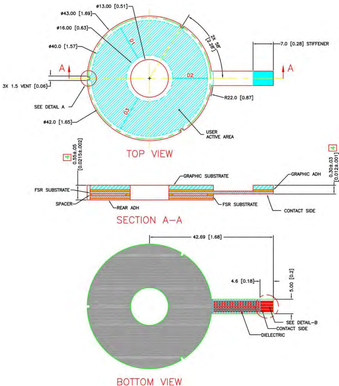
Figure 10: Ring Sensor
