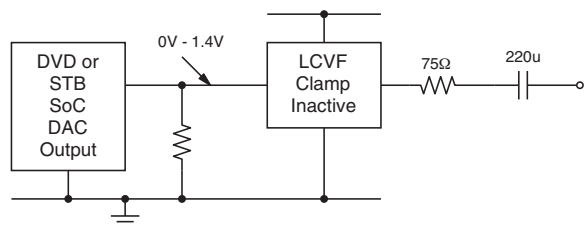
Figure 15. DC-coupled Inputs, AC-coupled Outputs
