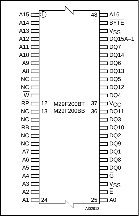
Figure 4. TSOP Connections
