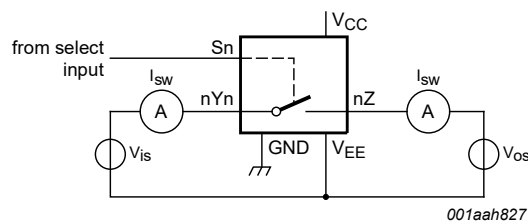
Fig. 9. Test circuit for measuring OFF-state current
