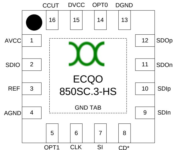
Figure 2: EQCO850SC-HS (EQCO875SC-HS ) Pin Layout (viewed from top) 2
