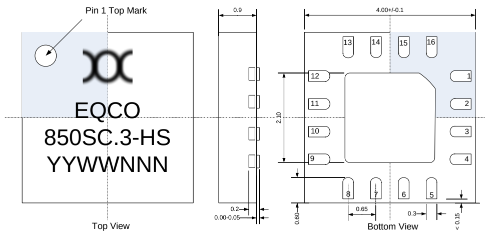
Figure 6: Package Drawings
