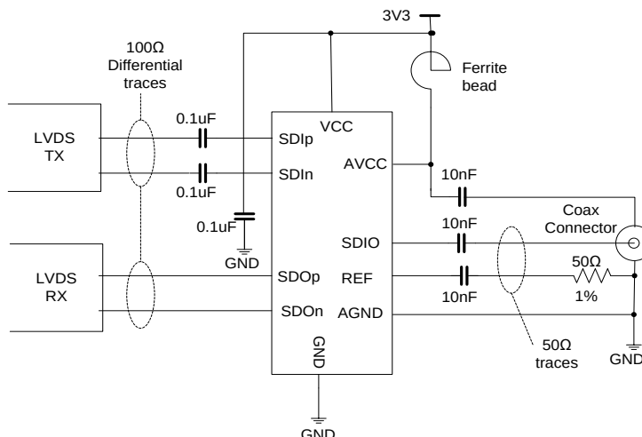
Figure 8: Example Schematic Implementation for EQCO850SC-HS.
