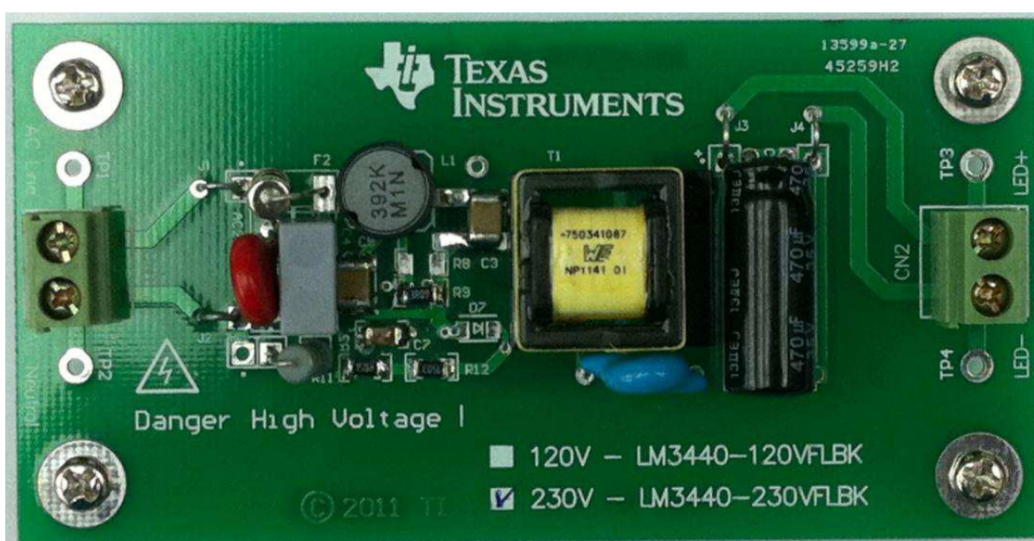
Figure 3. TPS92310EVM_8W
