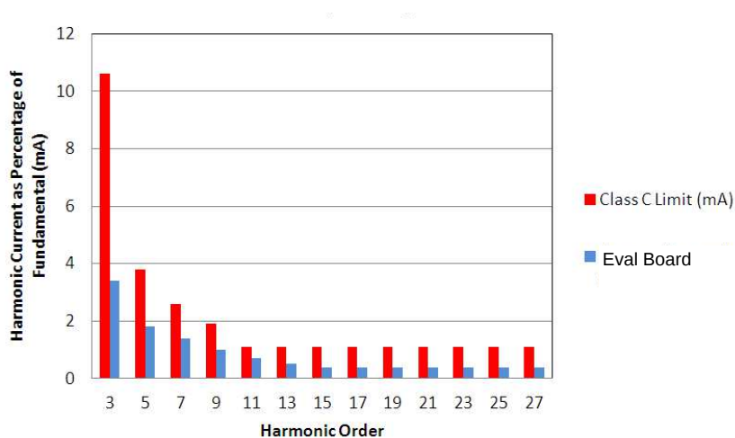
Figure 18. TPS92310 120V EVM Current Harmonic vs IEC61000-3-2 Class C Limits
