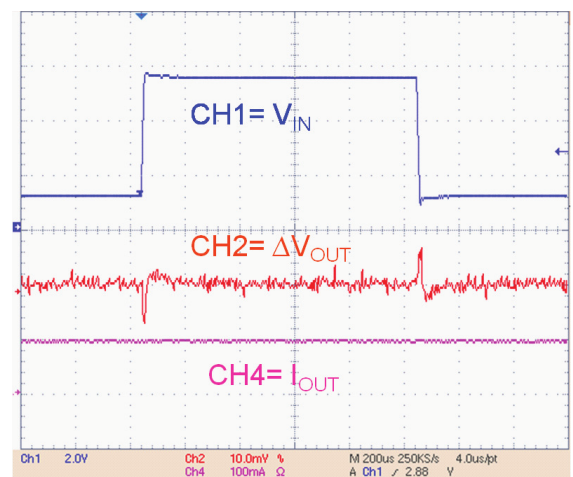
Figure 22. V_{IN} line transient
