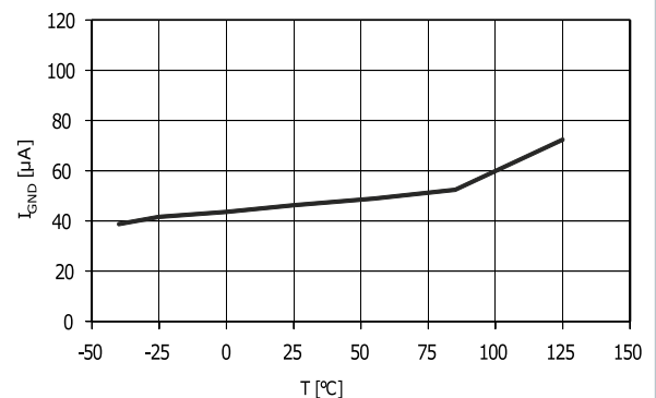
Figure 13. Ground current vs. temperature (adjustable, I_{OUT} = 800 \text{ mA} )
