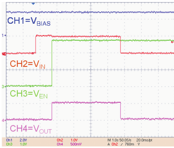
Figure 26. Enable transient, V_{BIAS} before V_{IN}
