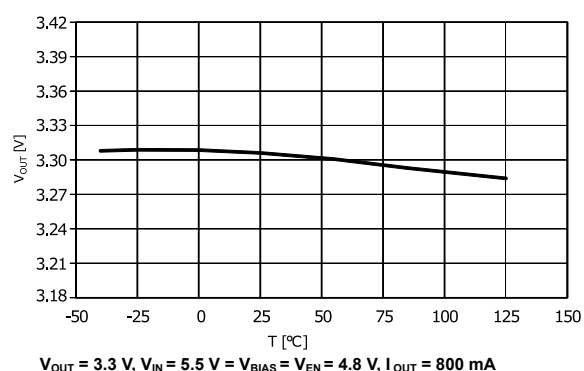
Figure 7. Output voltage vs. temperature (fixed 3.3 V, I_{OUT} = 800\text{ mA} )
