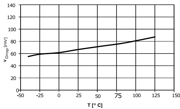
Figure 16. Dropout voltage vs. temperature (adjustable)
