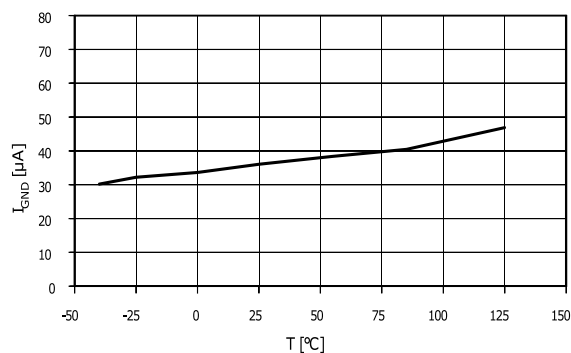
Figure 12. Ground current vs. temperature (adjustable, I_{OUT} = 500 \text{ mA} )
