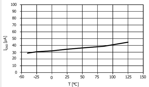
Figure 11. Ground current vs. temperature (adjustable, I_{OUT} = 0 \text{ mA} )
